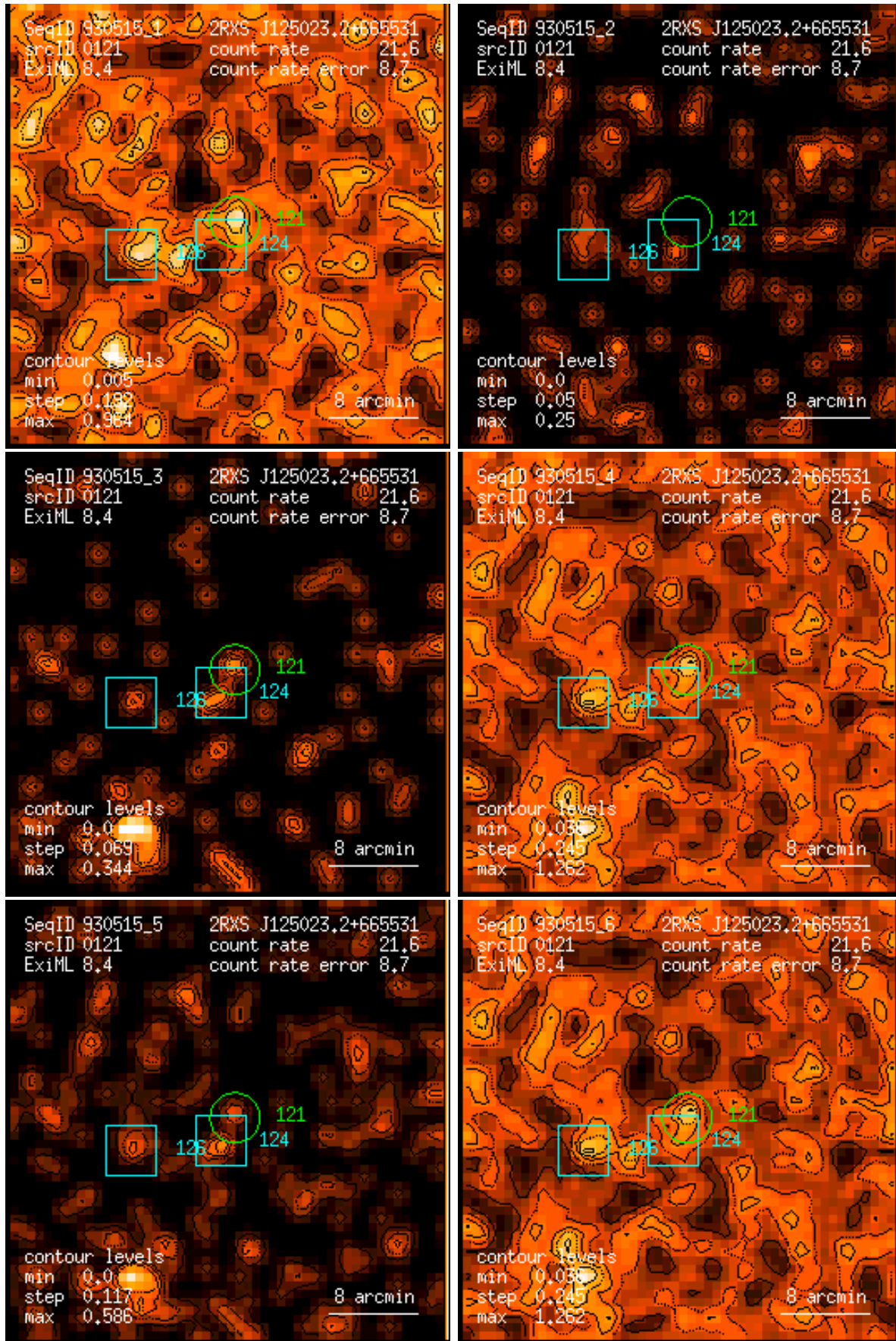
Figure 121: RASS 930515: detection 0121: band rate images, Gaussian filter: (1) PSPC channels 11 – 41, (2) 52 – 90, (3) 91 – 201, (4) 11 – 235, (5) 52 – 201, (6) 11 – 201. Broad band rates in counts/ks. Band rate contour levels in counts/ks/arcmin 2 .
