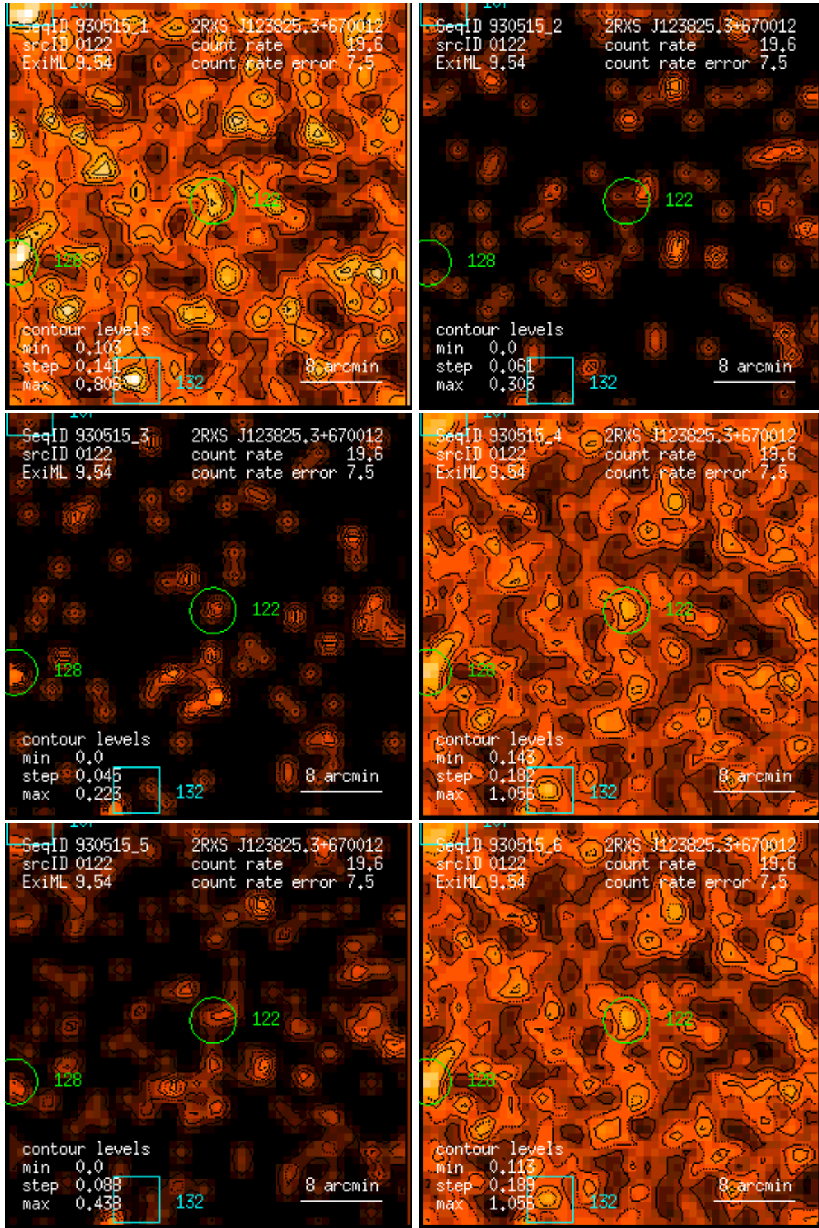
Figure 122: RASS 930515: detection 0122: band rate images, Gaussian filter: (1) PSPC channels 11 – 41, (2) 52 – 90, (3) 91 – 201, (4) 11 – 235, (5) 52 – 201, (6) 11 – 201. Broad band rates in counts/ks. Band rate contour levels in counts/ks/arcmin 2 .
