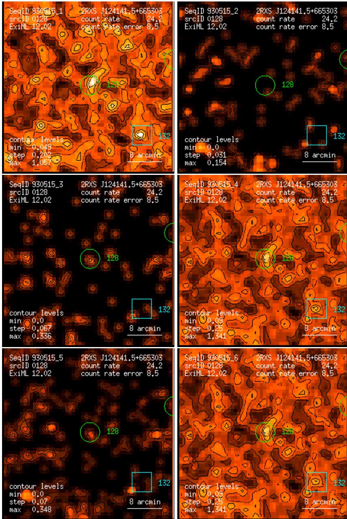
Figure 128: RASS 930515: detection 0128: band rate images, Gaussian filter: (1) PSPC channels 11 – 41, (2) 52 – 90, (3) 91 – 201, (4) 11 – 235, (5) 52 – 201, (6) 11 – 201. Broad band rates in counts/ks. Band rate contour levels in counts/ks/arcmin 2 .
