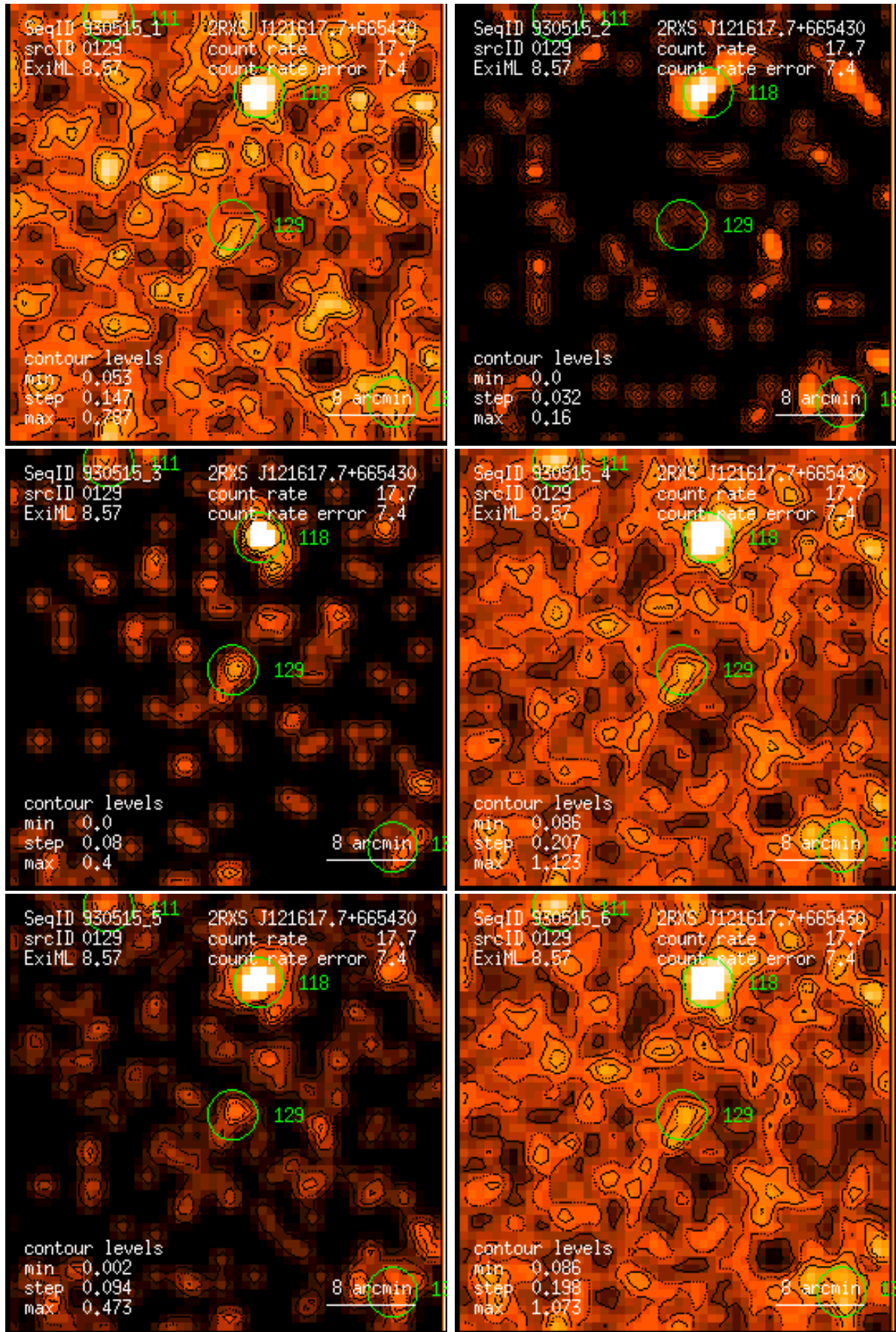
Figure 129: RASS 930515: detection 0129: band rate images, Gaussian filter: (1) PSPC channels 11 – 41, (2) 52 – 90, (3) 91 – 201, (4) 11 – 235, (5) 52 – 201, (6) 11 – 201. Broad band rates in counts/ks. Band rate contour levels in counts/ks/arcmin 2 .
