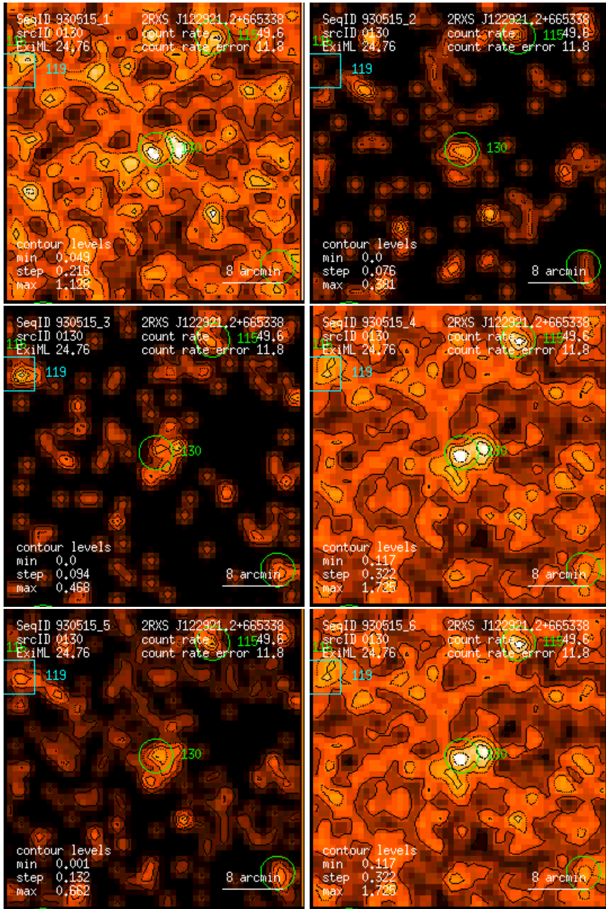
Figure 130: RASS 930515: detection 0130: band rate images, Gaussian filter: (1) PSPC channels 11 – 41, (2) 52 – 90, (3) 91 – 201, (4) 11 – 235, (5) 52 – 201, (6) 11 – 201. Broad band rates in counts/ks. Band rate contour levels in counts/ks/arcmin 2 .
