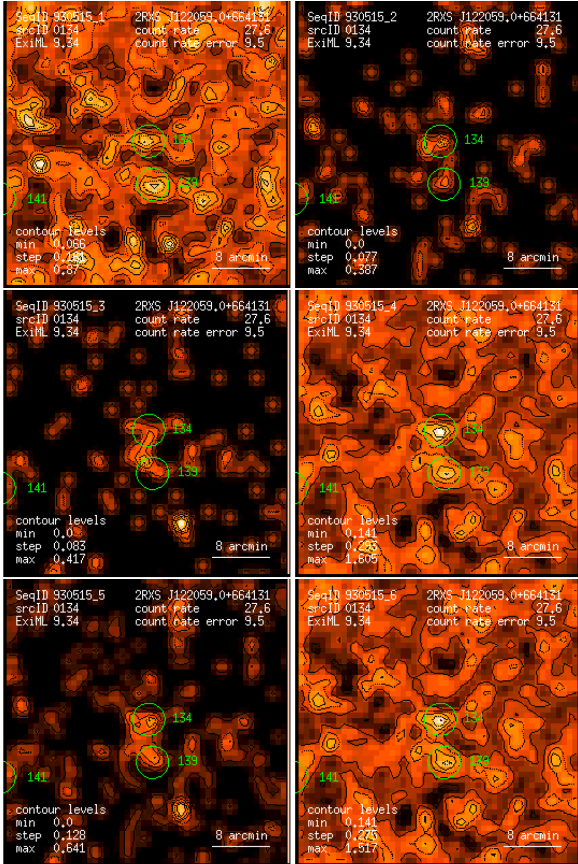
Figure 134: RASS 930515: detection 0134: band rate images, Gaussian filter: (1) PSPC channels 11 – 41, (2) 52 – 90, (3) 91 – 201, (4) 11 – 235, (5) 52 – 201, (6) 11 – 201. Broad band rates in counts/ks. Band rate contour levels in counts/ks/arcmin 2 .
