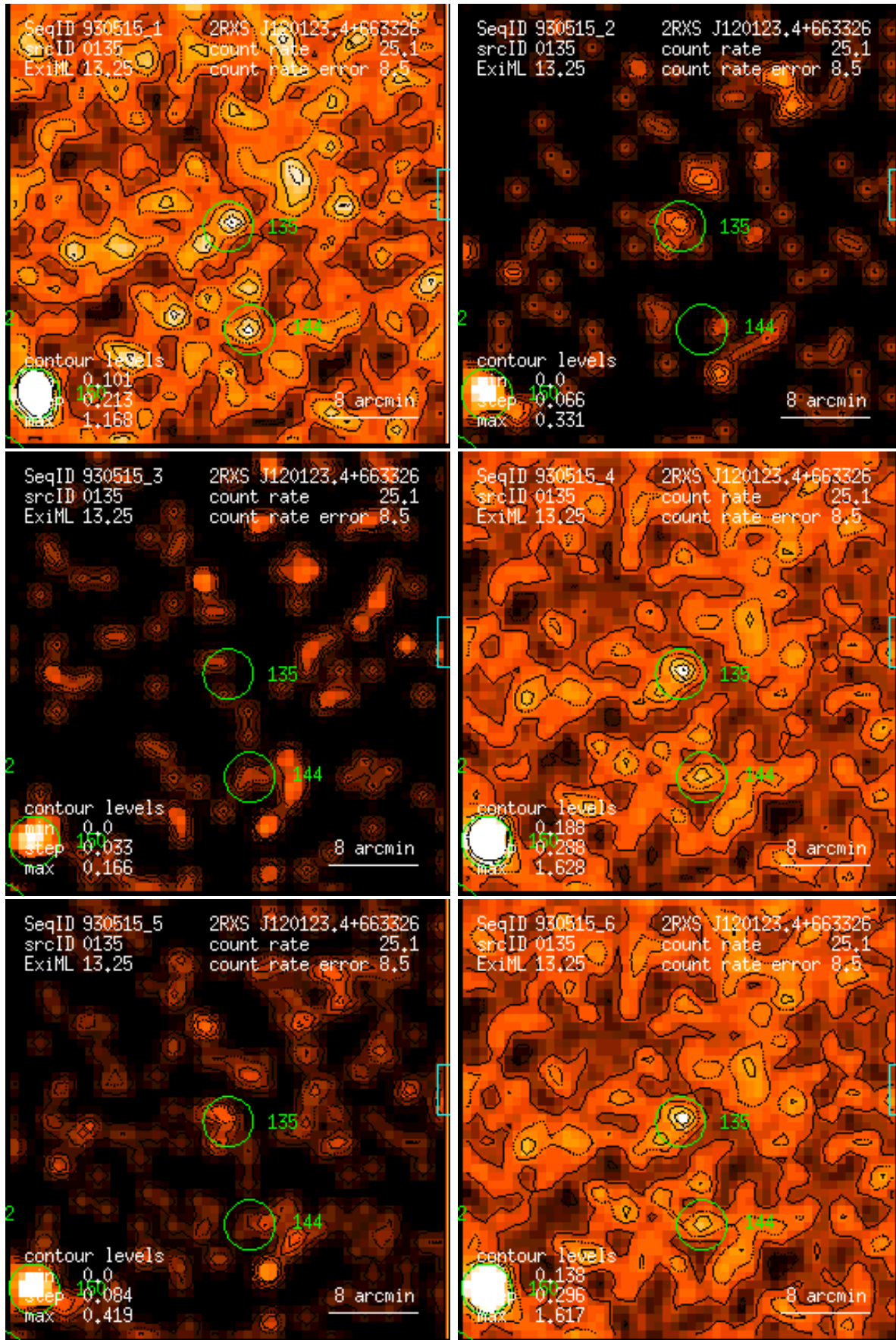
Figure 135: RASS 930515: detection 0135: band rate images, Gaussian filter: (1) PSPC channels 11 – 41, (2) 52 – 90, (3) 91 – 201, (4) 11 – 235, (5) 52 – 201, (6) 11 – 201. Broad band rates in counts/ks. Band rate contour levels in counts/ks/arcmin 2 .
