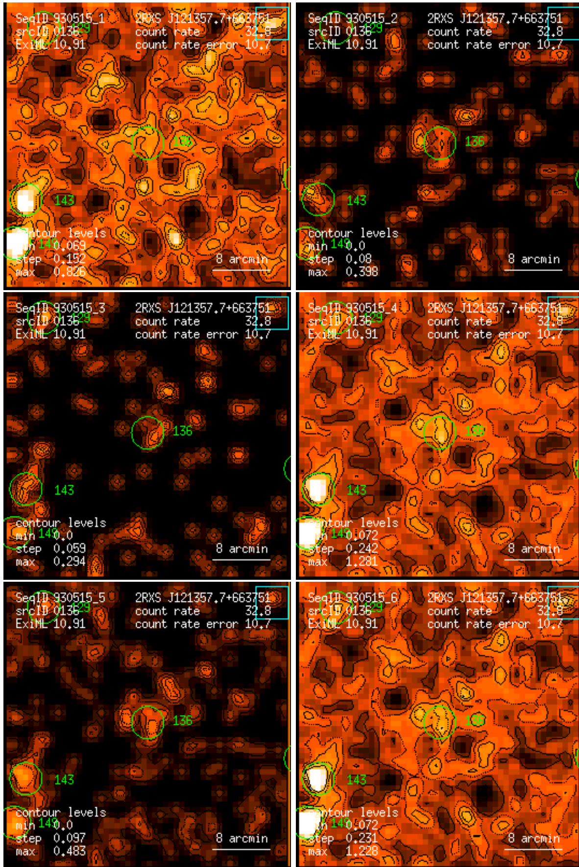
Figure 136: RASS 930515: detection 0136: band rate images, Gaussian filter: (1) PSPC channels 11 – 41, (2) 52 – 90, (3) 91 – 201, (4) 11 – 235, (5) 52 – 201, (6) 11 – 201. Broad band rates in counts/ks. Band rate contour levels in counts/ks/arcmin 2 .
