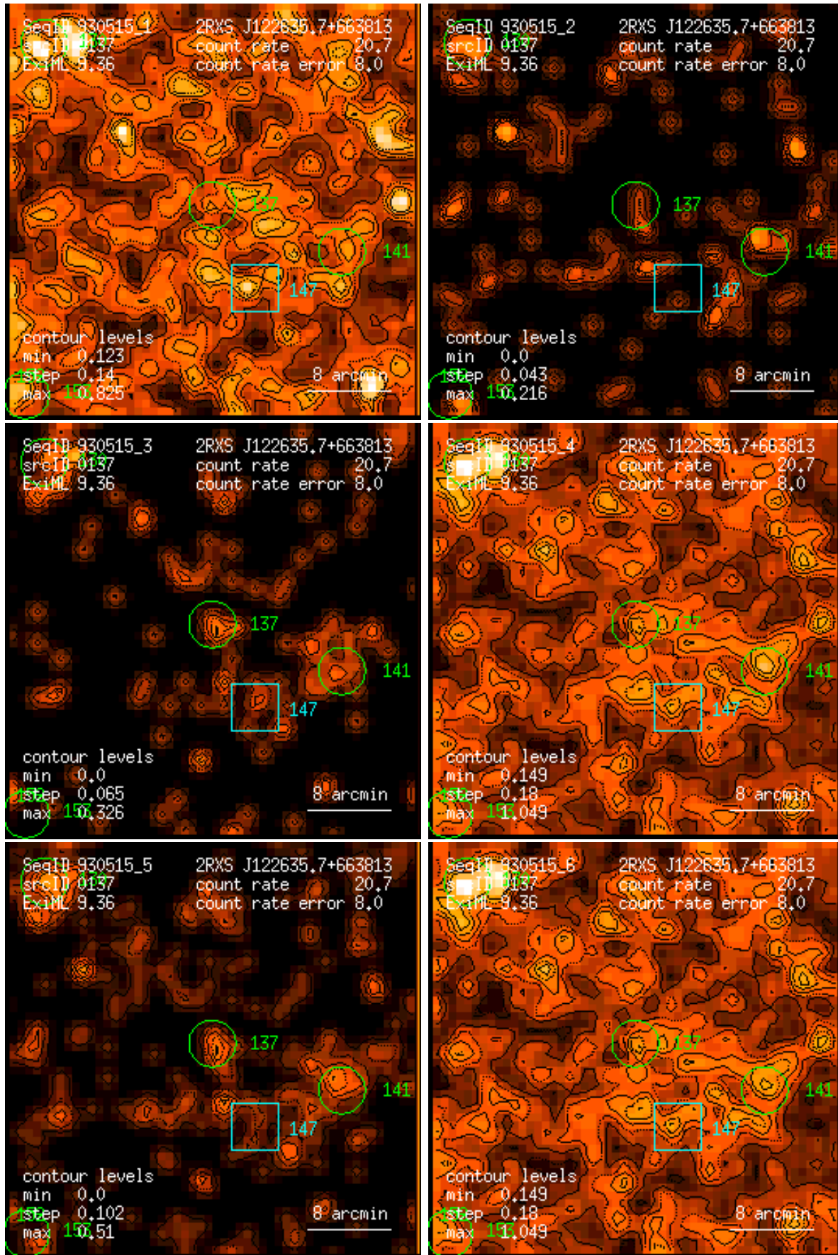
Figure 137: RASS 930515: detection 0137: band rate images, Gaussian filter: (1) PSPC channels 11 – 41, (2) 52 – 90, (3) 91 – 201, (4) 11 – 235, (5) 52 – 201, (6) 11 – 201. Broad band rates in counts/ks. Band rate contour levels in counts/ks/arcmin 2 .
