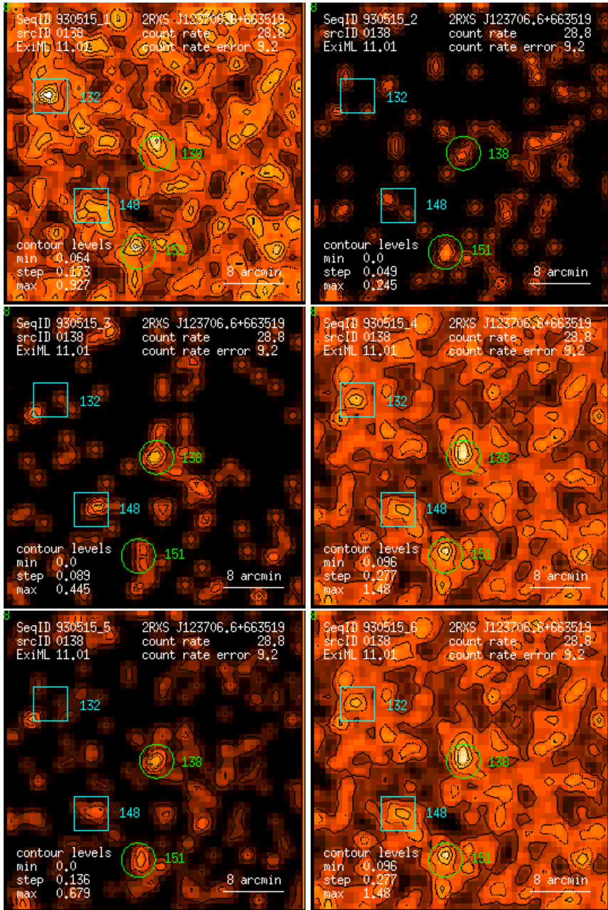
Figure 138: RASS 930515: detection 0138: band rate images, Gaussian filter: (1) PSPC channels 11 – 41, (2) 52 – 90, (3) 91 – 201, (4) 11 – 235, (5) 52 – 201, (6) 11 – 201. Broad band rates in counts/ks. Band rate contour levels in counts/ks/arcmin 2 .
