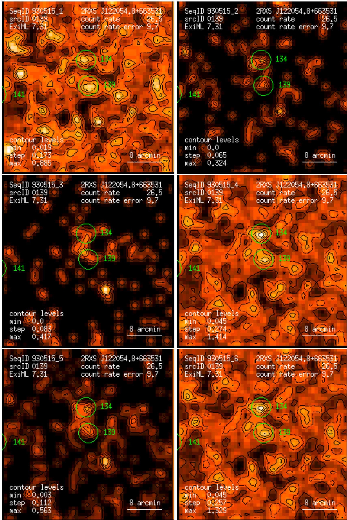
Figure 139: RASS 930515: detection 0139: band rate images, Gaussian filter: (1) PSPC channels 11 – 41, (2) 52 – 90, (3) 91 – 201, (4) 11 – 235, (5) 52 – 201, (6) 11 – 201. Broad band rates in counts/ks. Band rate contour levels in counts/ks/arcmin 2 .
