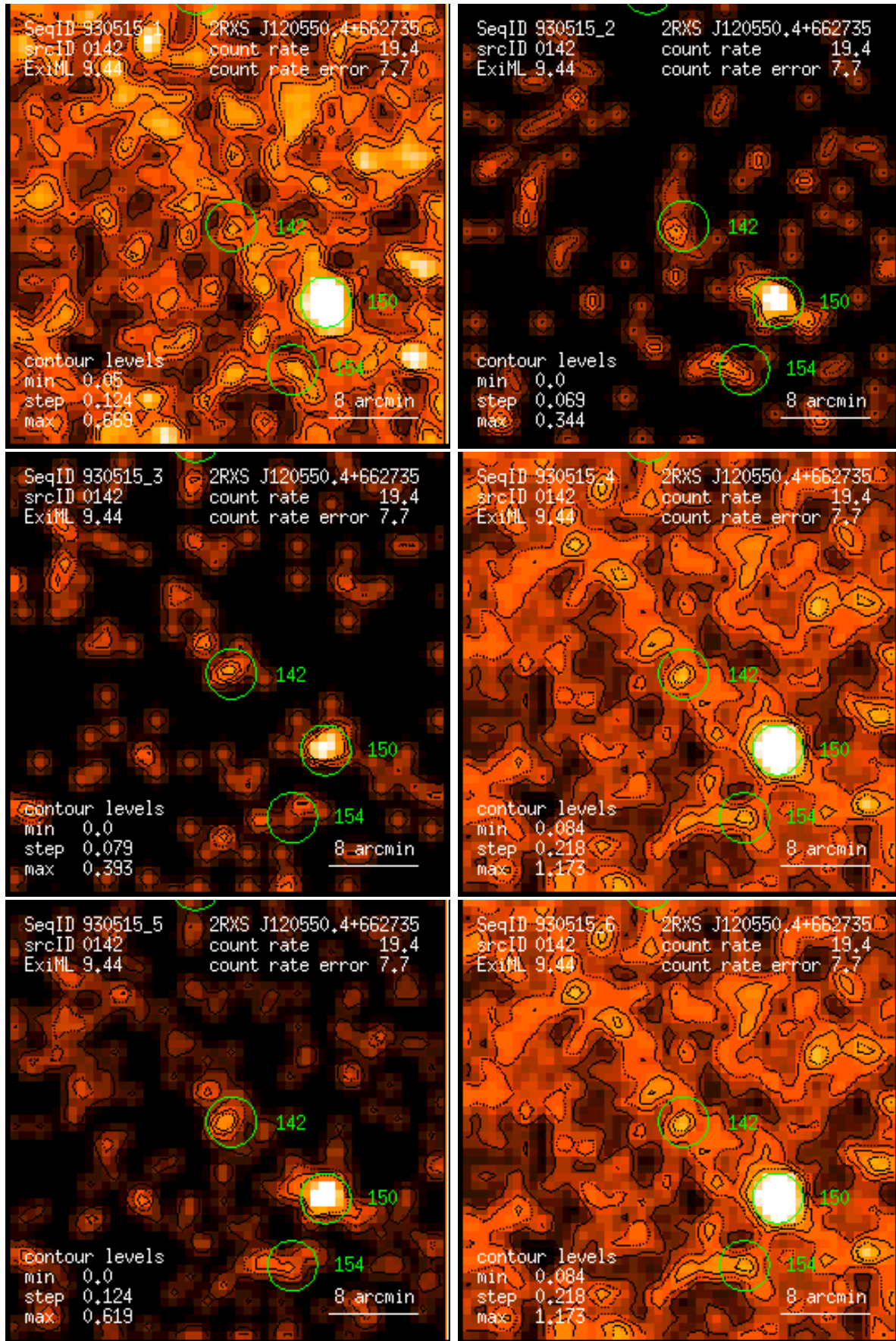
Figure 142: RASS 930515: detection 0142: band rate images, Gaussian filter: (1) PSPC channels 11 – 41, (2) 52 – 90, (3) 91 – 201, (4) 11 – 235, (5) 52 – 201, (6) 11 – 201. Broad band rates in counts/ks. Band rate contour levels in counts/ks/arcmin 2 .
