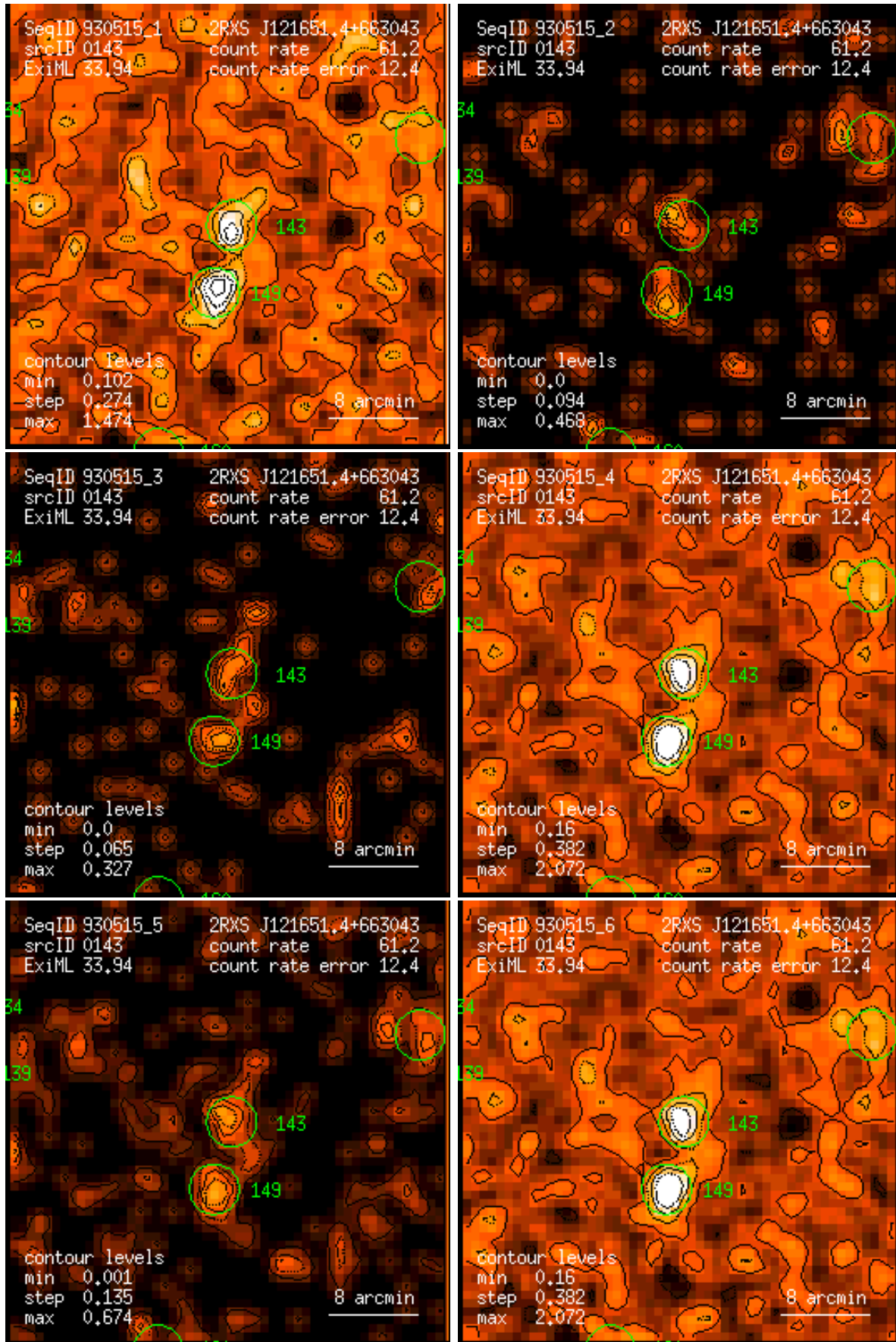
Figure 143: RASS 930515: detection 0143: band rate images, Gaussian filter: (1) PSPC channels 11 – 41, (2) 52 – 90, (3) 91 – 201, (4) 11 – 235, (5) 52 – 201, (6) 11 – 201. Broad band rates in counts/ks. Band rate contour levels in counts/ks/arcmin 2 .
