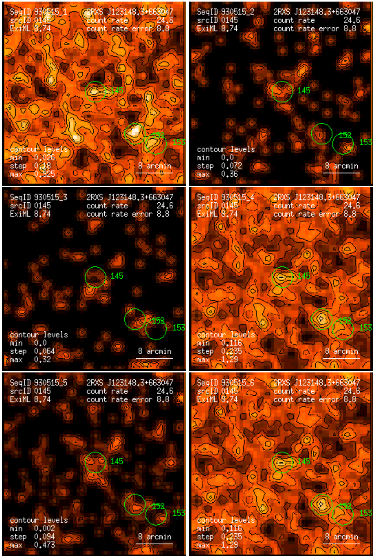
Figure 145: RASS 930515: detection 0145: band rate images, Gaussian filter: (1) PSPC channels 11 – 41, (2) 52 – 90, (3) 91 – 201, (4) 11 – 235, (5) 52 – 201, (6) 11 – 201. Broad band rates in counts/ks. Band rate contour levels in counts/ks/arcmin 2 .
