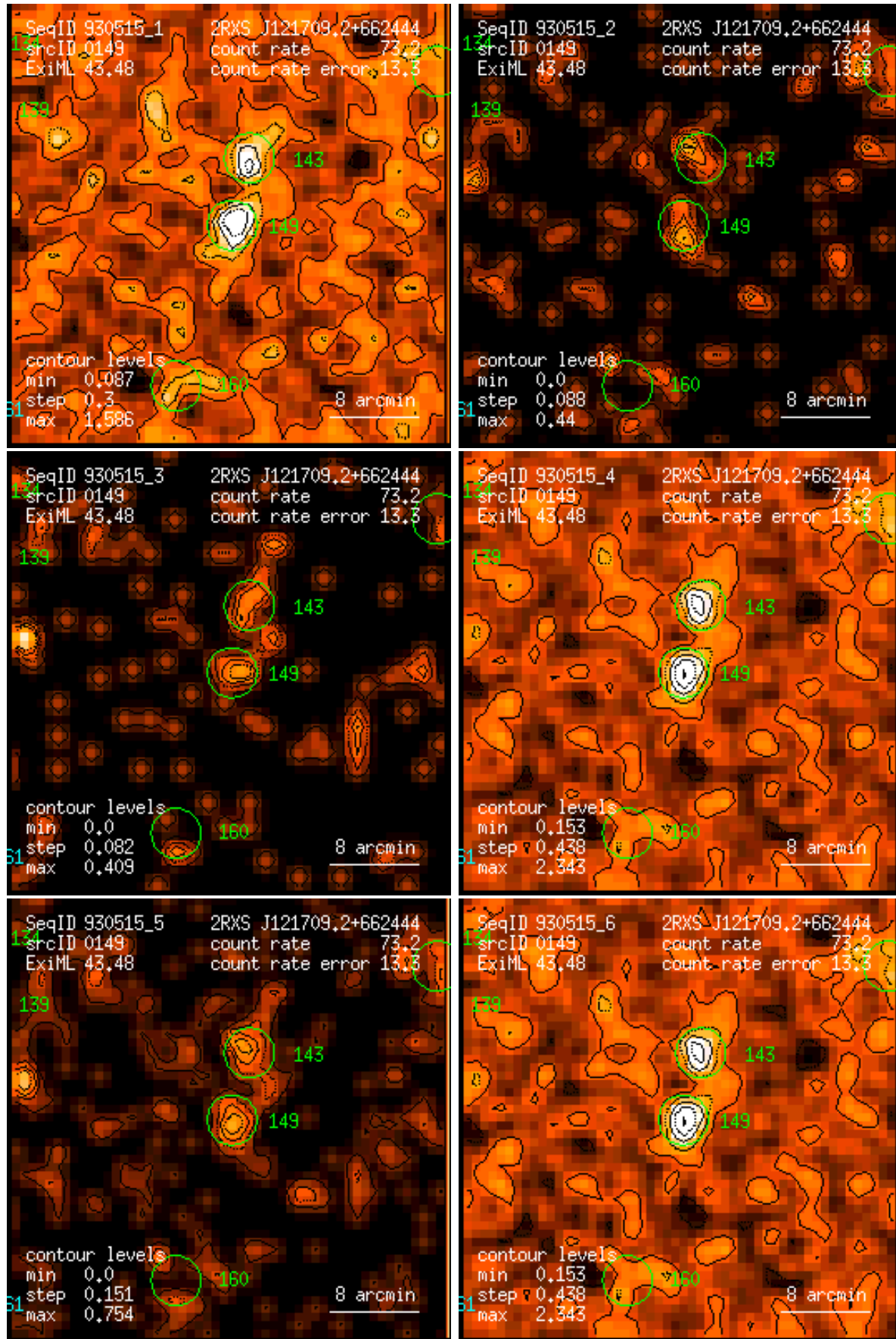
Figure 149: RASS 930515: detection 0149: band rate images, Gaussian filter: (1) PSPC channels 11 – 41, (2) 52 – 90, (3) 91 – 201, (4) 11 – 235, (5) 52 – 201, (6) 11 – 201. Broad band rates in counts/ks. Band rate contour levels in counts/ks/arcmin 2 .
