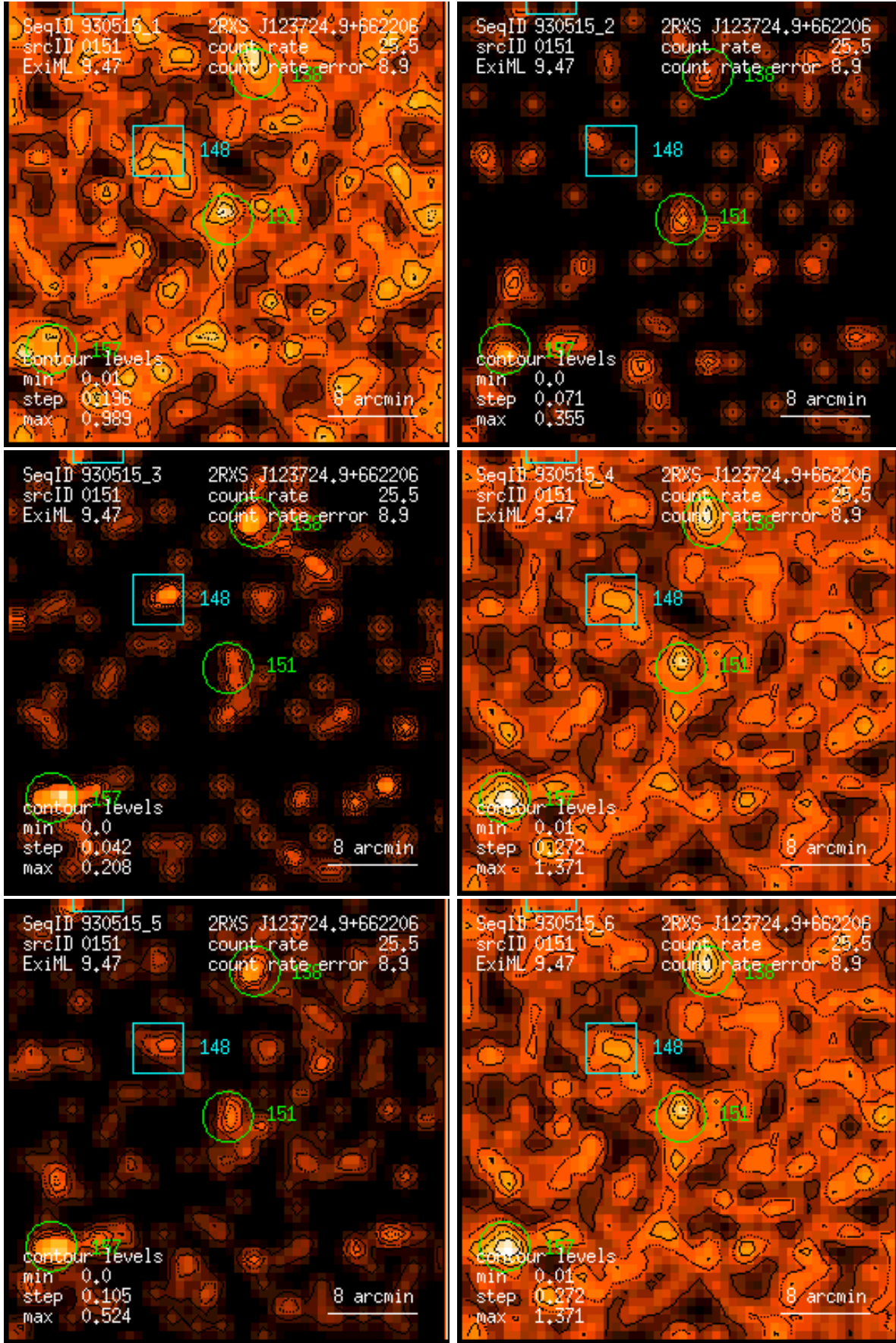
Figure 151: RASS 930515: detection 0151: band rate images, Gaussian filter: (1) PSPC channels 11 – 41, (2) 52 – 90, (3) 91 – 201, (4) 11 – 235, (5) 52 – 201, (6) 11 – 201. Broad band rates in counts/ks. Band rate contour levels in counts/ks/arcmin 2 .
