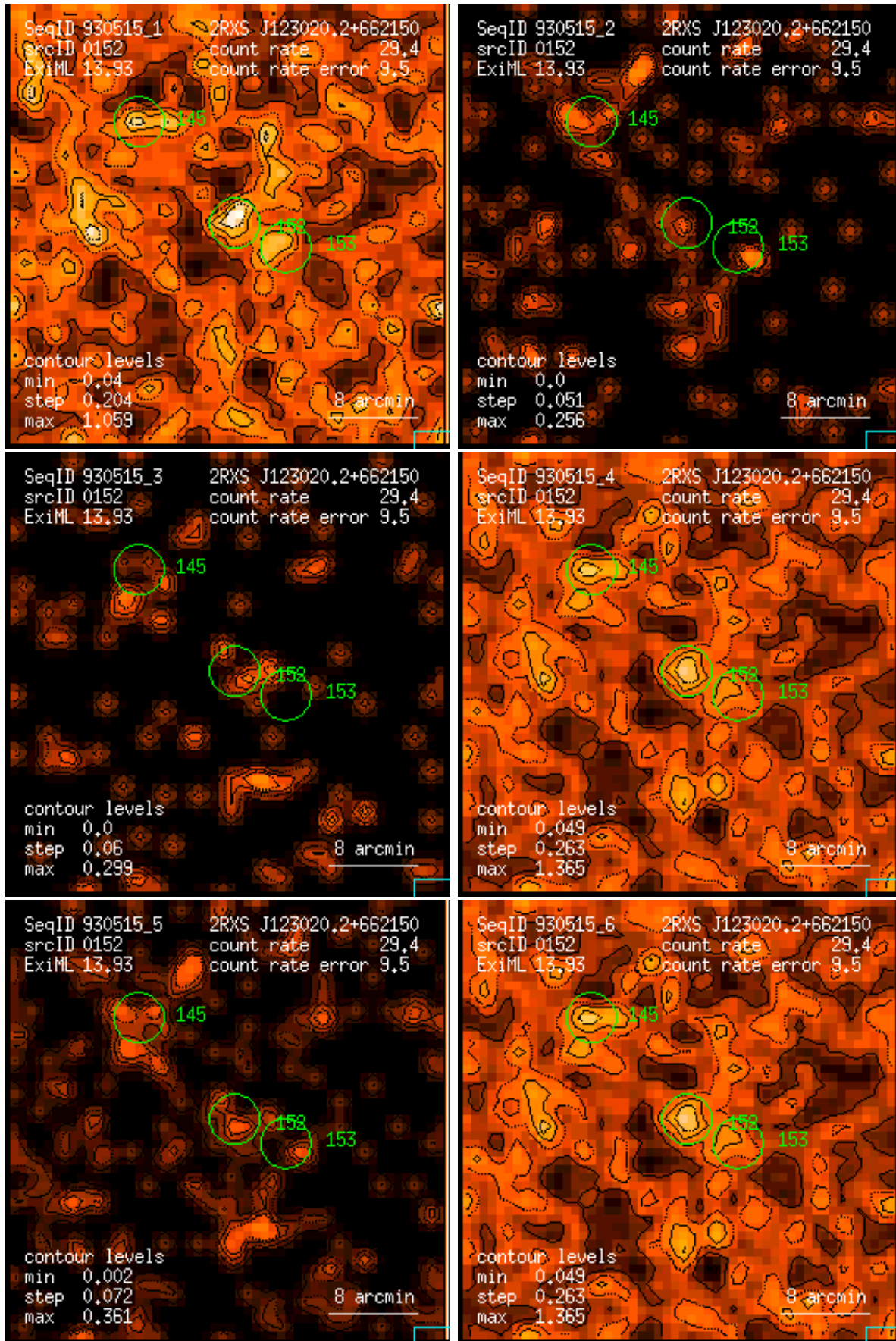
Figure 152: RASS 930515: detection 0152: band rate images, Gaussian filter: (1) PSPC channels 11 – 41, (2) 52 – 90, (3) 91 – 201, (4) 11 – 235, (5) 52 – 201, (6) 11 – 201. Broad band rates in counts/ks. Band rate contour levels in counts/ks/arcmin 2 .
