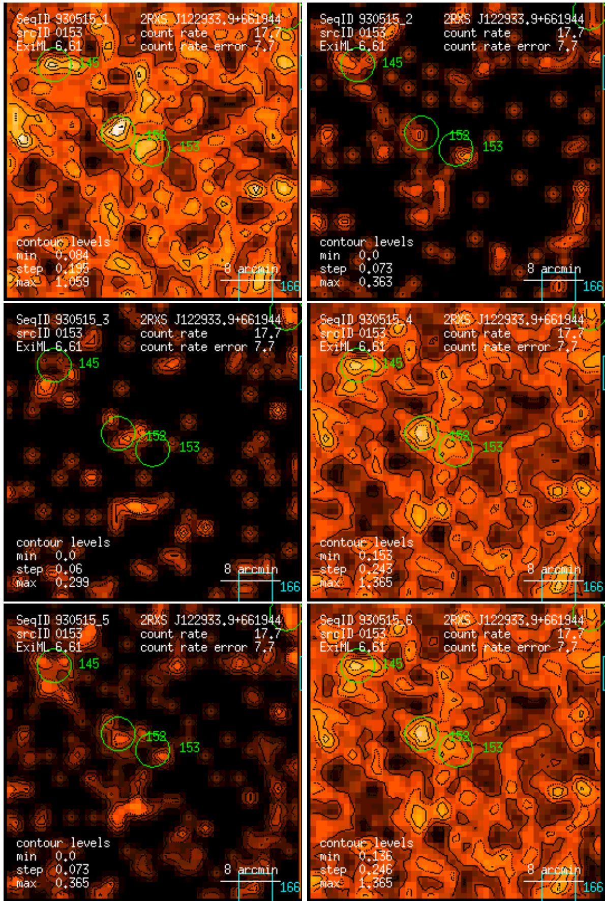
Figure 153: RASS 930515: detection 0153: band rate images, Gaussian filter: (1) PSPC channels 11 – 41, (2) 52 – 90, (3) 91 – 201, (4) 11 – 235, (5) 52 – 201, (6) 11 – 201. Broad band rates in counts/ks. Band rate contour levels in counts/ks/arcmin 2 .
