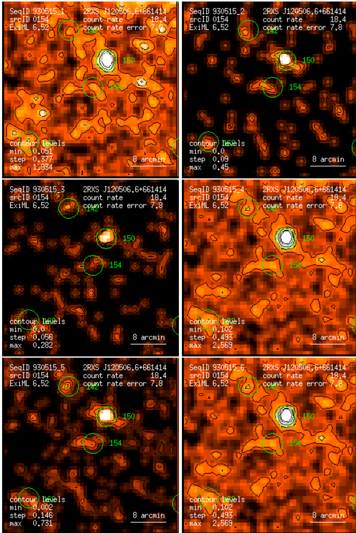
Figure 154: RASS 930515: detection 0154: band rate images, Gaussian filter: (1) PSPC channels 11 – 41, (2) 52 – 90, (3) 91 – 201, (4) 11 – 235, (5) 52 – 201, (6) 11 – 201. Broad band rates in counts/ks. Band rate contour levels in counts/ks/arcmin 2 .
