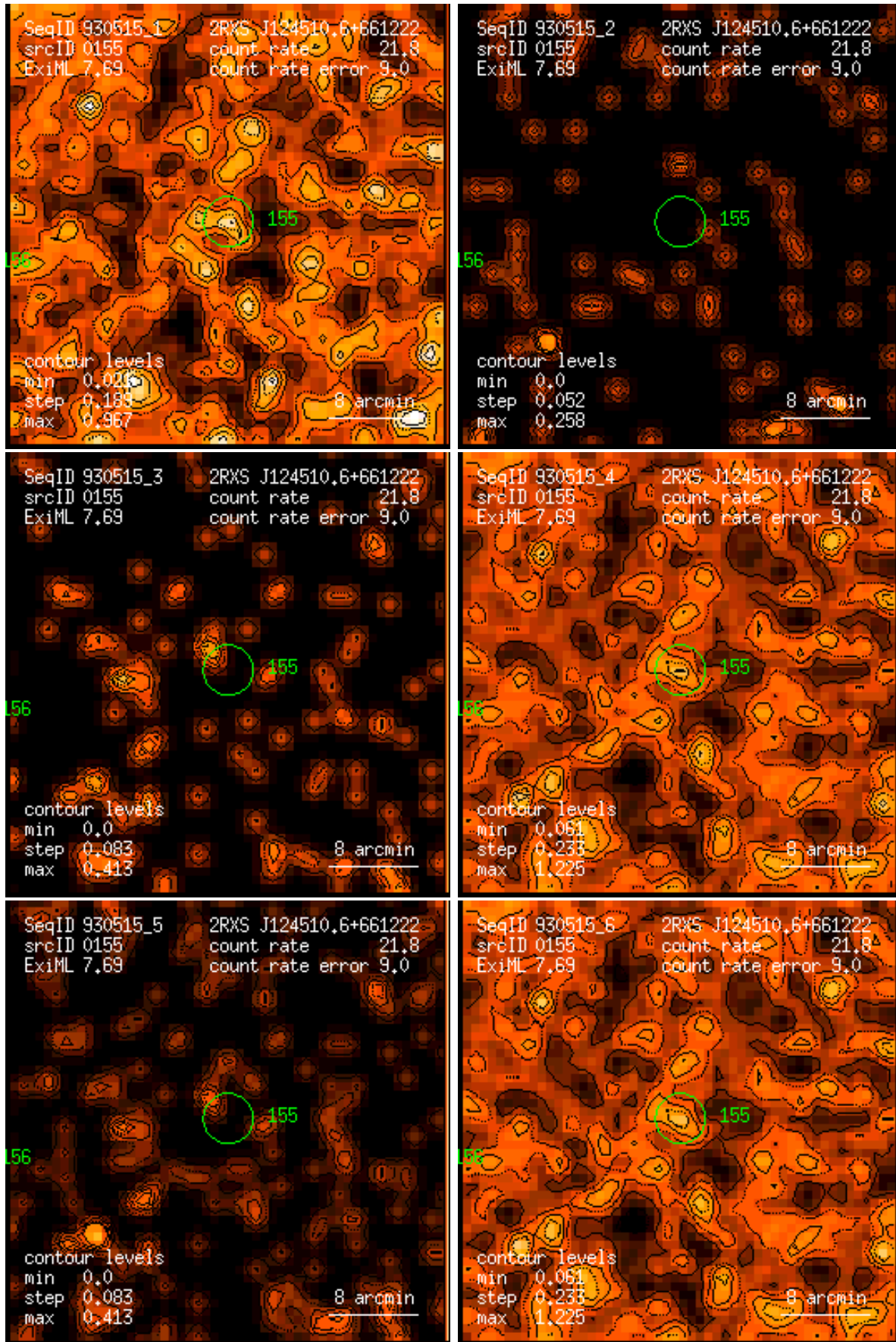
Figure 155: RASS 930515: detection 0155: band rate images, Gaussian filter: (1) PSPC channels 11 – 41, (2) 52 – 90, (3) 91 – 201, (4) 11 – 235, (5) 52 – 201, (6) 11 – 201. Broad band rates in counts/ks. Band rate contour levels in counts/ks/arcmin 2 .
