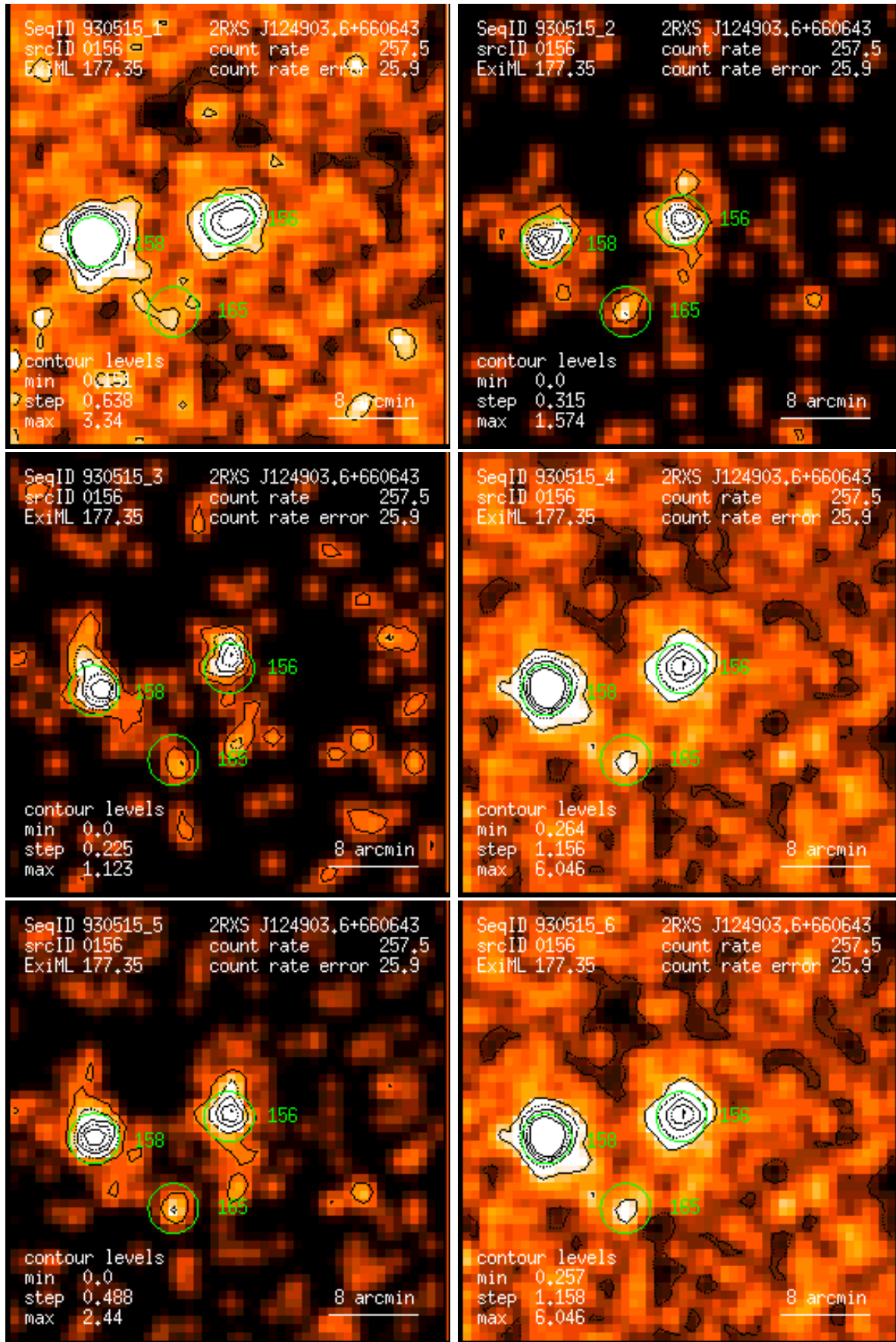
Figure 156: RASS 930515: detection 0156: band rate images, Gaussian filter: (1) PSPC channels 11 – 41, (2) 52 – 90, (3) 91 – 201, (4) 11 – 235, (5) 52 – 201, (6) 11 – 201. Broad band rates in counts/ks. Band rate contour levels in counts/ks/arcmin 2 .
