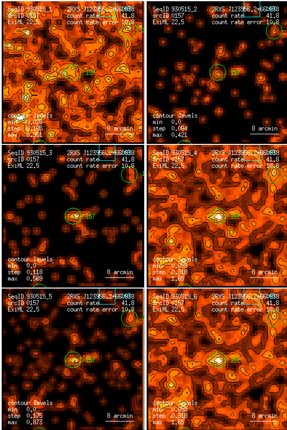
Figure 157: RASS 930515: detection 0157: band rate images, Gaussian filter: (1) PSPC channels 11 – 41, (2) 52 – 90, (3) 91 – 201, (4) 11 – 235, (5) 52 – 201, (6) 11 – 201. Broad band rates in counts/ks. Band rate contour levels in counts/ks/arcmin 2 .
