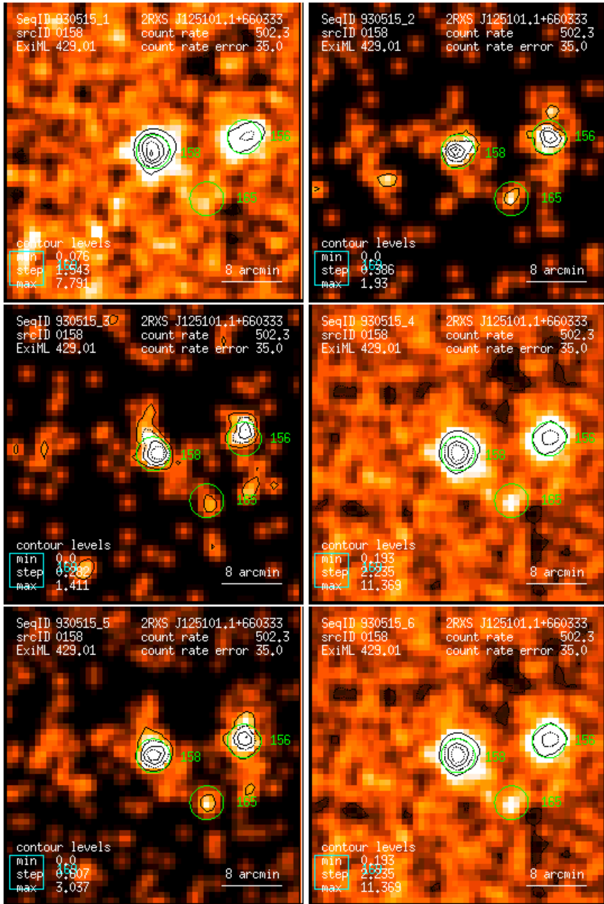
Figure 158: RASS 930515: detection 0158: band rate images, Gaussian filter: (1) PSPC channels 11 – 41, (2) 52 – 90, (3) 91 – 201, (4) 11 – 235, (5) 52 – 201, (6) 11 – 201. Broad band rates in counts/ks. Band rate contour levels in counts/ks/arcmin 2 .
