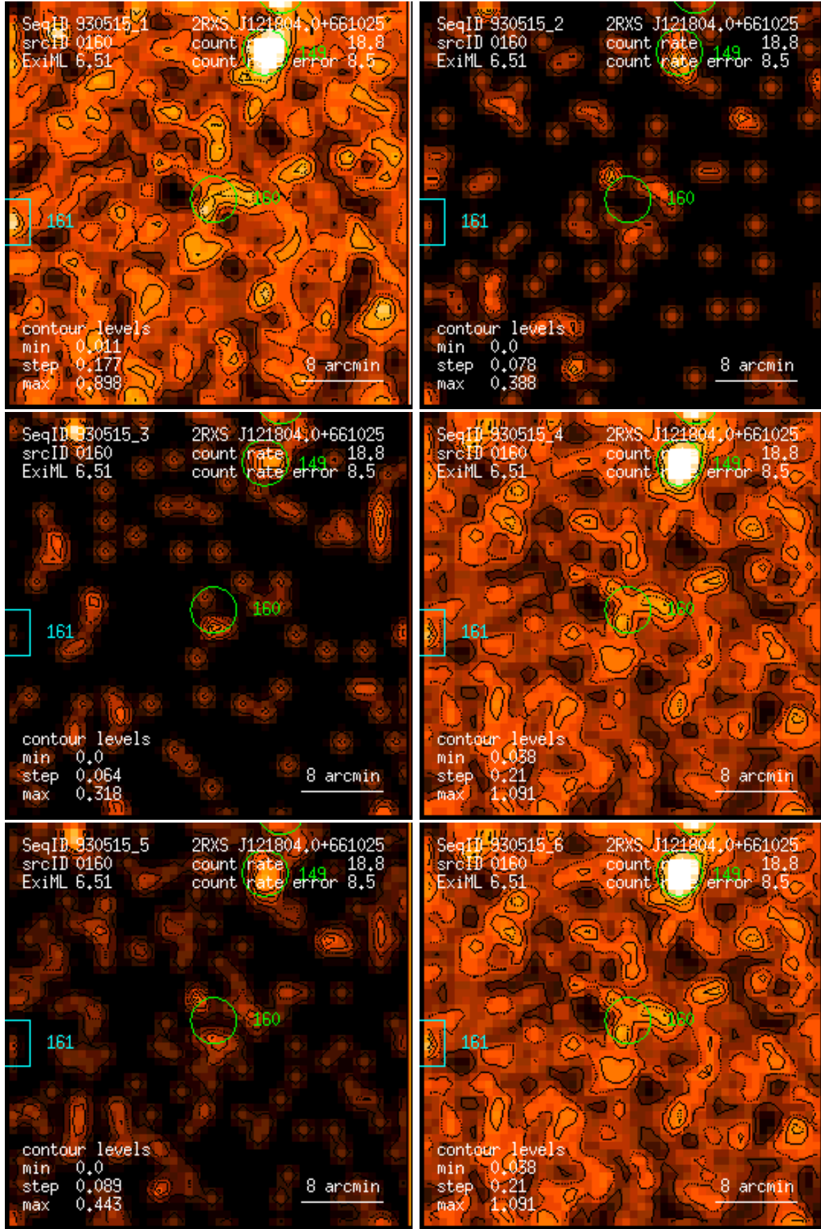
Figure 160: RASS 930515: detection 0160: band rate images, Gaussian filter: (1) PSPC channels 11 – 41, (2) 52 – 90, (3) 91 – 201, (4) 11 – 235, (5) 52 – 201, (6) 11 – 201. Broad band rates in counts/ks. Band rate contour levels in counts/ks/arcmin 2 .
