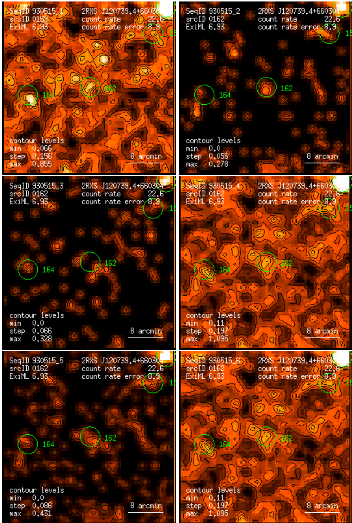
Figure 162: RASS 930515: detection 0162: band rate images, Gaussian filter: (1) PSPC channels 11 – 41, (2) 52 – 90, (3) 91 – 201, (4) 11 – 235, (5) 52 – 201, (6) 11 – 201. Broad band rates in counts/ks. Band rate contour levels in counts/ks/arcmin 2 .
