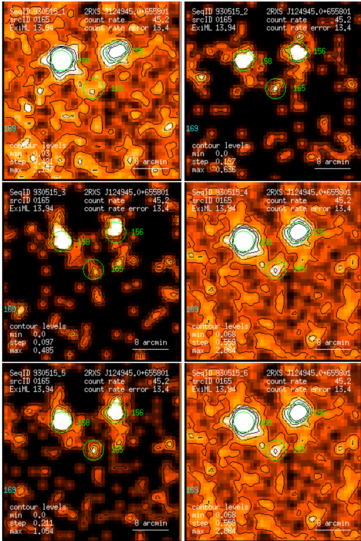
Figure 165: RASS 930515: detection 0165: band rate images, Gaussian filter: (1) PSPC channels 11 – 41, (2) 52 – 90, (3) 91 – 201, (4) 11 – 235, (5) 52 – 201, (6) 11 – 201. Broad band rates in counts/ks. Band rate contour levels in counts/ks/arcmin 2 .
