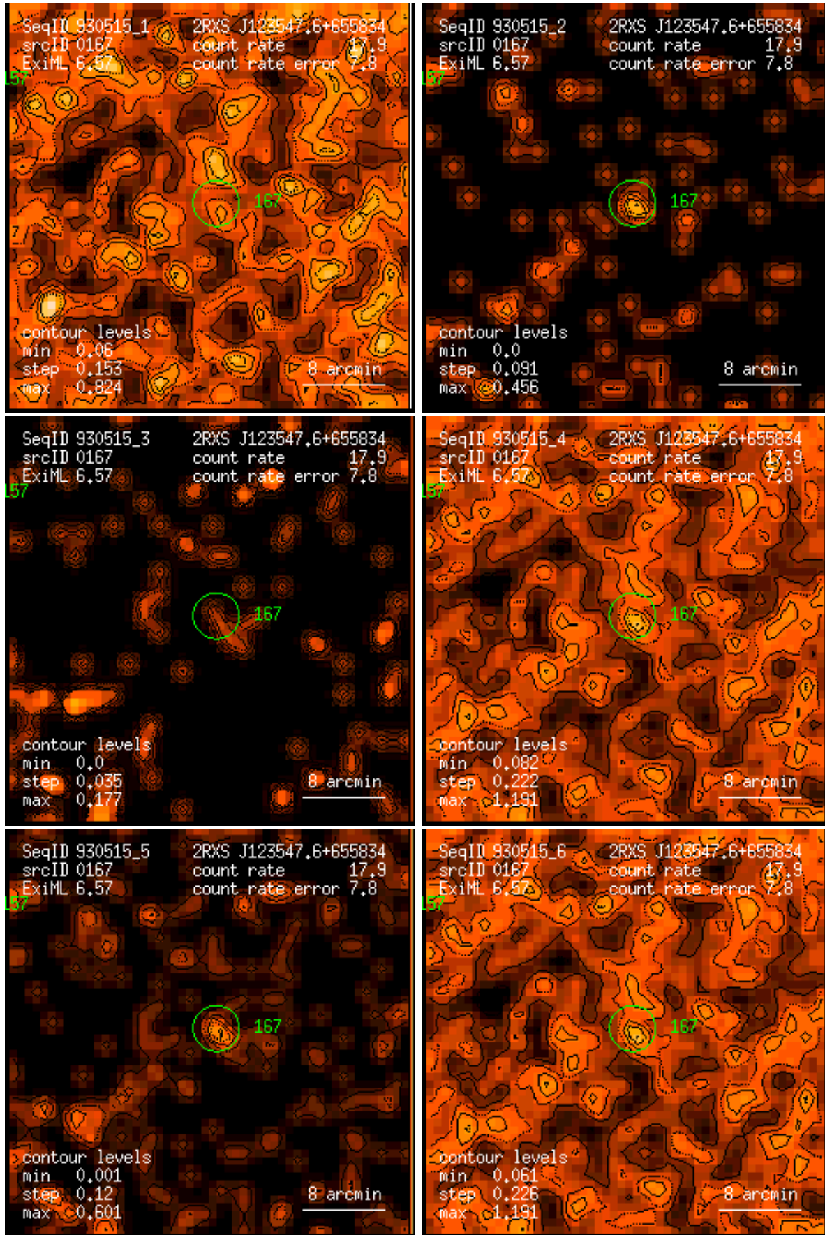
Figure 167: RASS 930515: detection 0167: band rate images, Gaussian filter: (1) PSPC channels 11 – 41, (2) 52 – 90, (3) 91 – 201, (4) 11 – 235, (5) 52 – 201, (6) 11 – 201. Broad band rates in counts/ks. Band rate contour levels in counts/ks/arcmin 2 .
