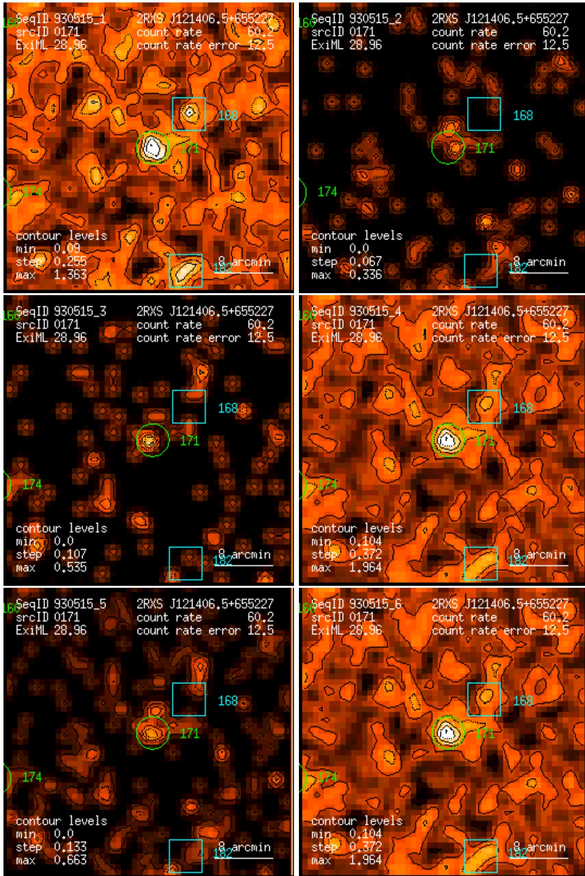
Figure 171: RASS 930515: detection 0171: band rate images, Gaussian filter: (1) PSPC channels 11 – 41, (2) 52 – 90, (3) 91 – 201, (4) 11 – 235, (5) 52 – 201, (6) 11 – 201. Broad band rates in counts/ks. Band rate contour levels in counts/ks/arcmin 2 .
