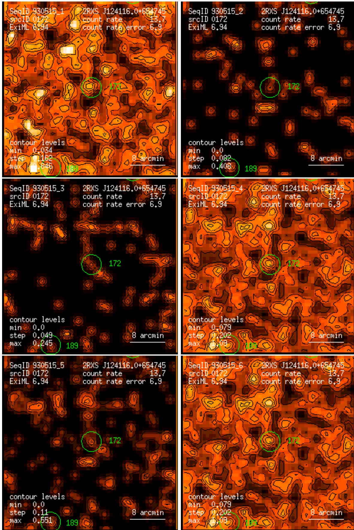
Figure 172: RASS 930515: detection 0172: band rate images, Gaussian filter: (1) PSPC channels 11 – 41, (2) 52 – 90, (3) 91 – 201, (4) 11 – 235, (5) 52 – 201, (6) 11 – 201. Broad band rates in counts/ks. Band rate contour levels in counts/ks/arcmin 2 .
