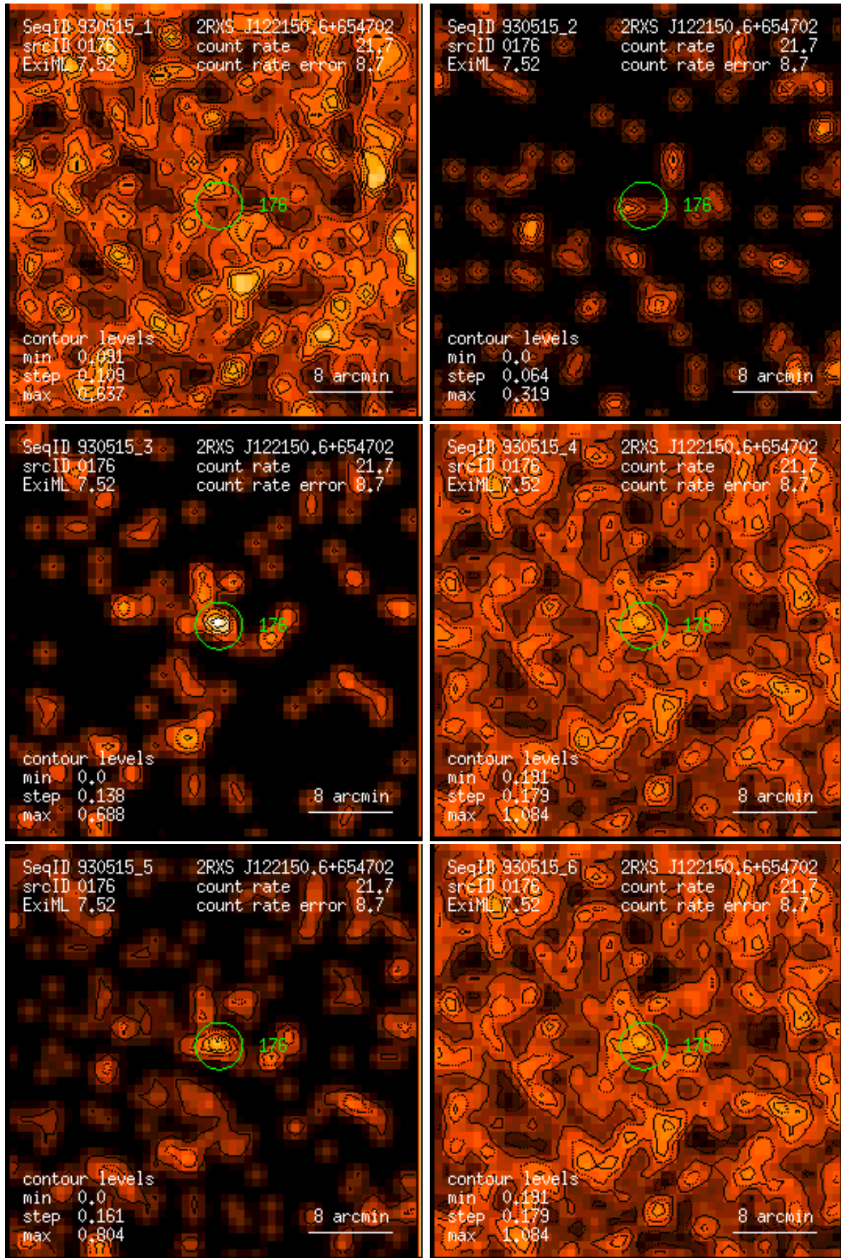
Figure 176: RASS 930515: detection 0176: band rate images, Gaussian filter: (1) PSPC channels 11 – 41, (2) 52 – 90, (3) 91 – 201, (4) 11 – 235, (5) 52 – 201, (6) 11 – 201. Broad band rates in counts/ks. Band rate contour levels in counts/ks/arcmin 2 .
