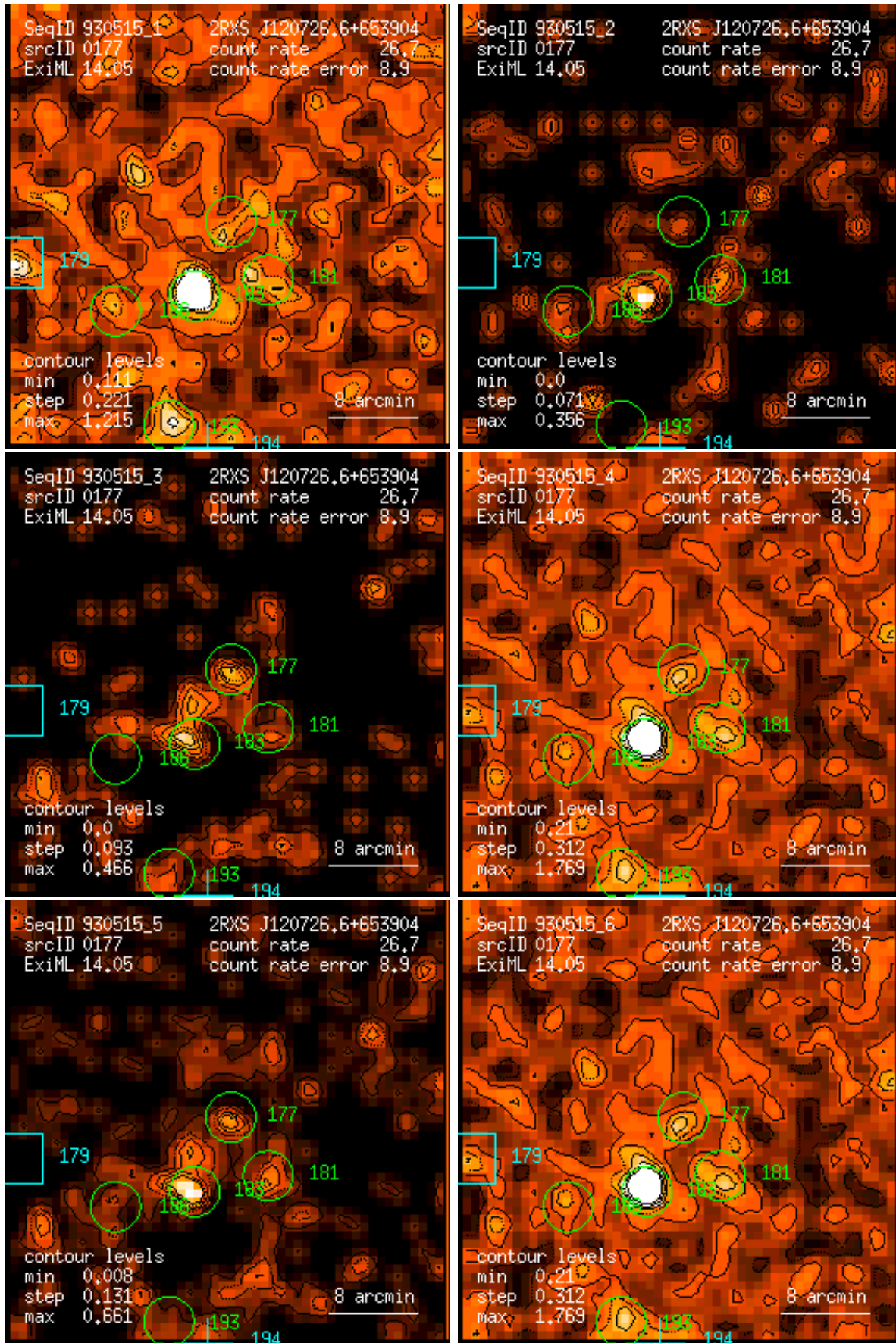
Figure 177: RASS 930515: detection 0177: band rate images, Gaussian filter: (1) PSPC channels 11 – 41, (2) 52 – 90, (3) 91 – 201, (4) 11 – 235, (5) 52 – 201, (6) 11 – 201. Broad band rates in counts/ks. Band rate contour levels in counts/ks/arcmin 2 .
