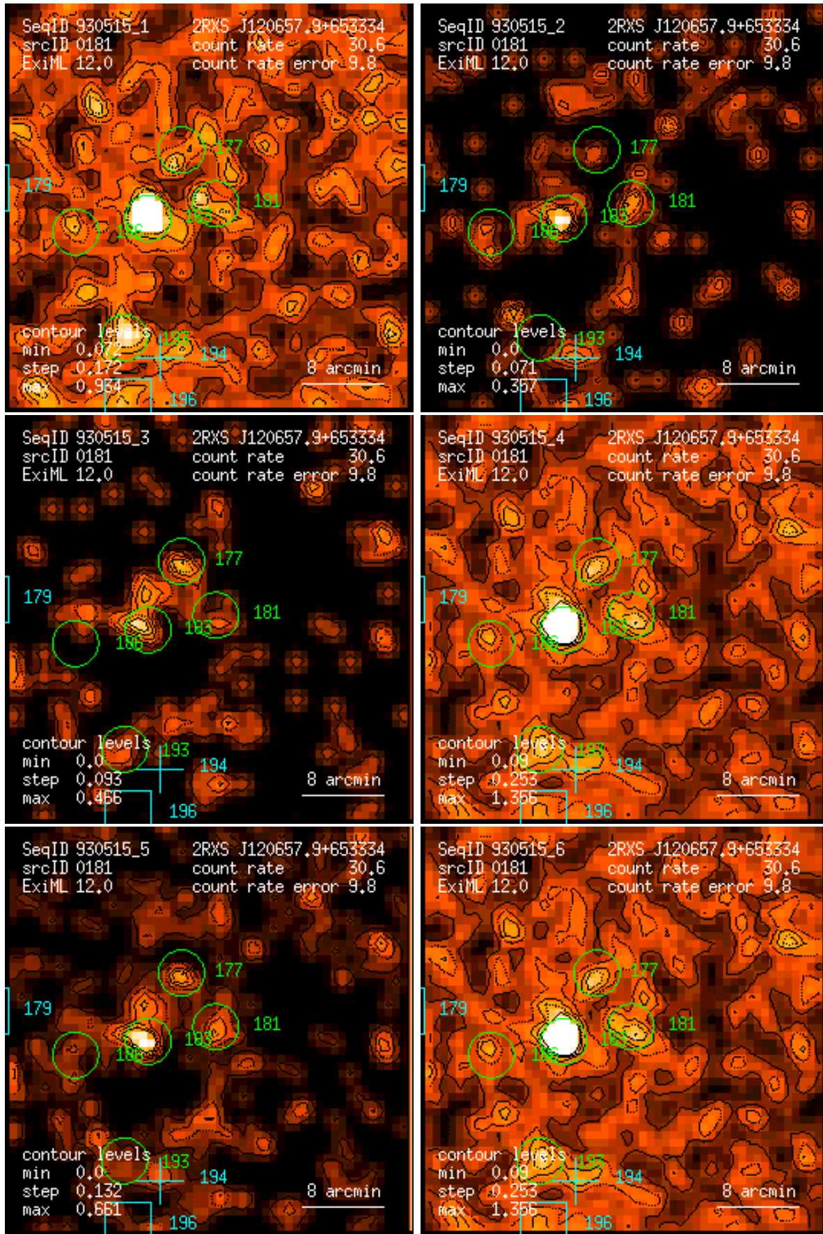
Figure 181: RASS 930515: detection 0181: band rate images, Gaussian filter: (1) PSPC channels 11 – 41, (2) 52 – 90, (3) 91 – 201, (4) 11 – 235, (5) 52 – 201, (6) 11 – 201. Broad band rates in counts/ks. Band rate contour levels in counts/ks/arcmin 2 .
