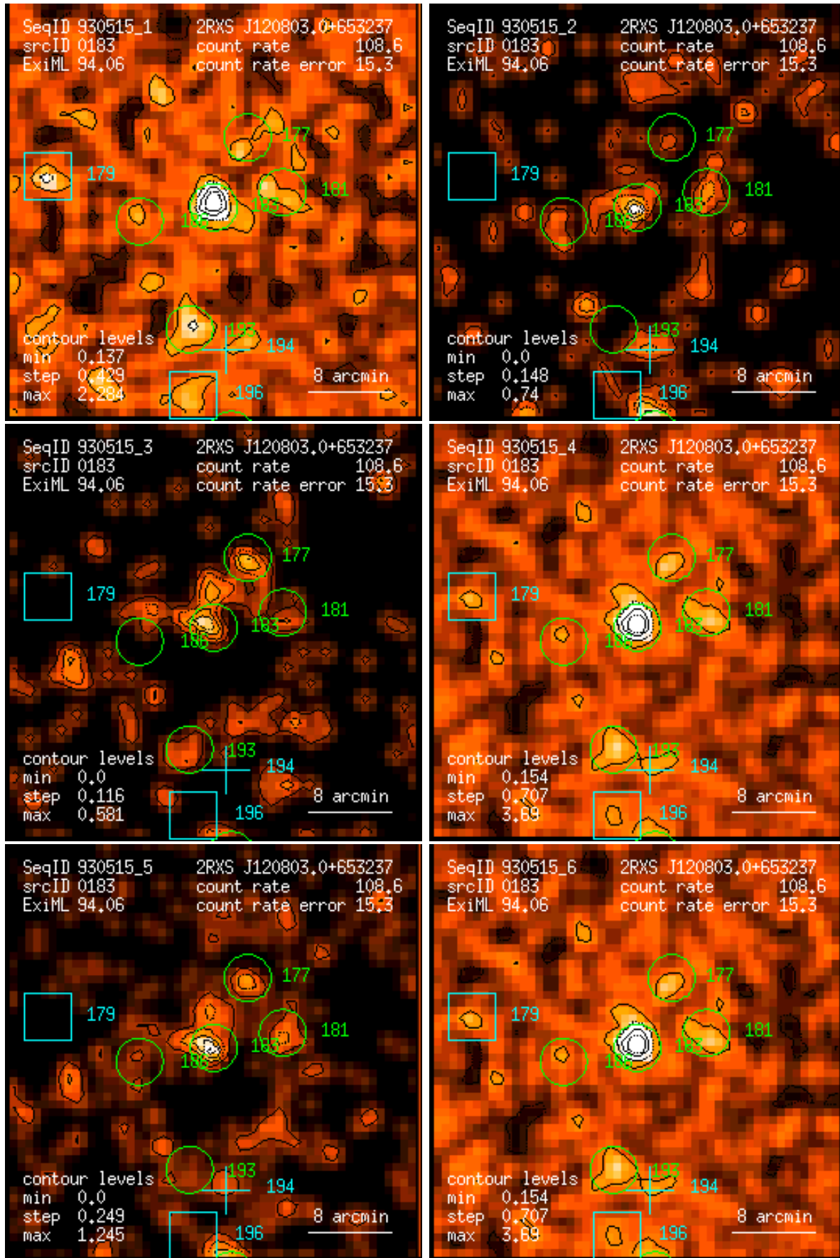
Figure 183: RASS 930515: detection 0183: band rate images, Gaussian filter: (1) PSPC channels 11 – 41, (2) 52 – 90, (3) 91 – 201, (4) 11 – 235, (5) 52 – 201, (6) 11 – 201. Broad band rates in counts/ks. Band rate contour levels in counts/ks/arcmin 2 .
