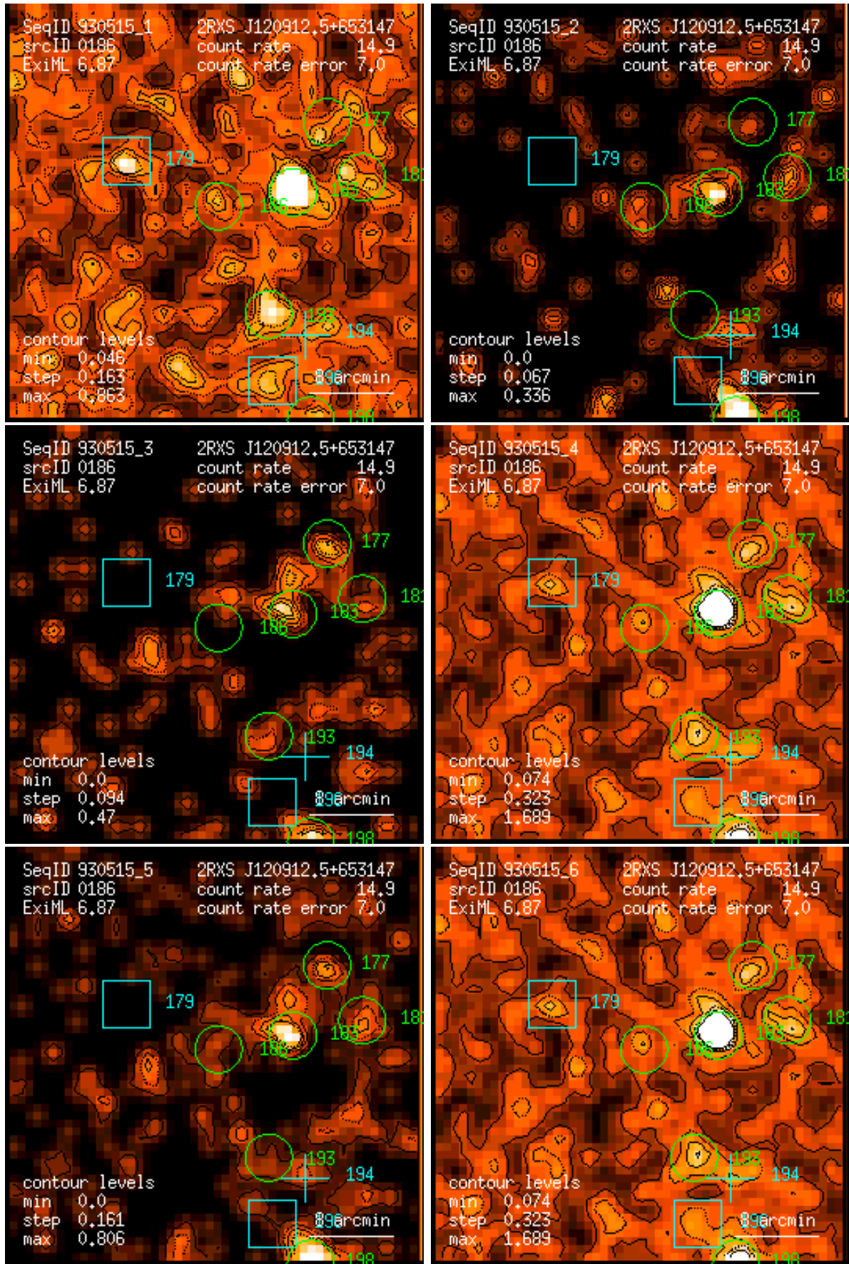
Figure 186: RASS 930515: detection 0186: band rate images, Gaussian filter: (1) PSPC channels 11 – 41, (2) 52 – 90, (3) 91 – 201, (4) 11 – 235, (5) 52 – 201, (6) 11 – 201. Broad band rates in counts/ks. Band rate contour levels in counts/ks/arcmin 2 .
