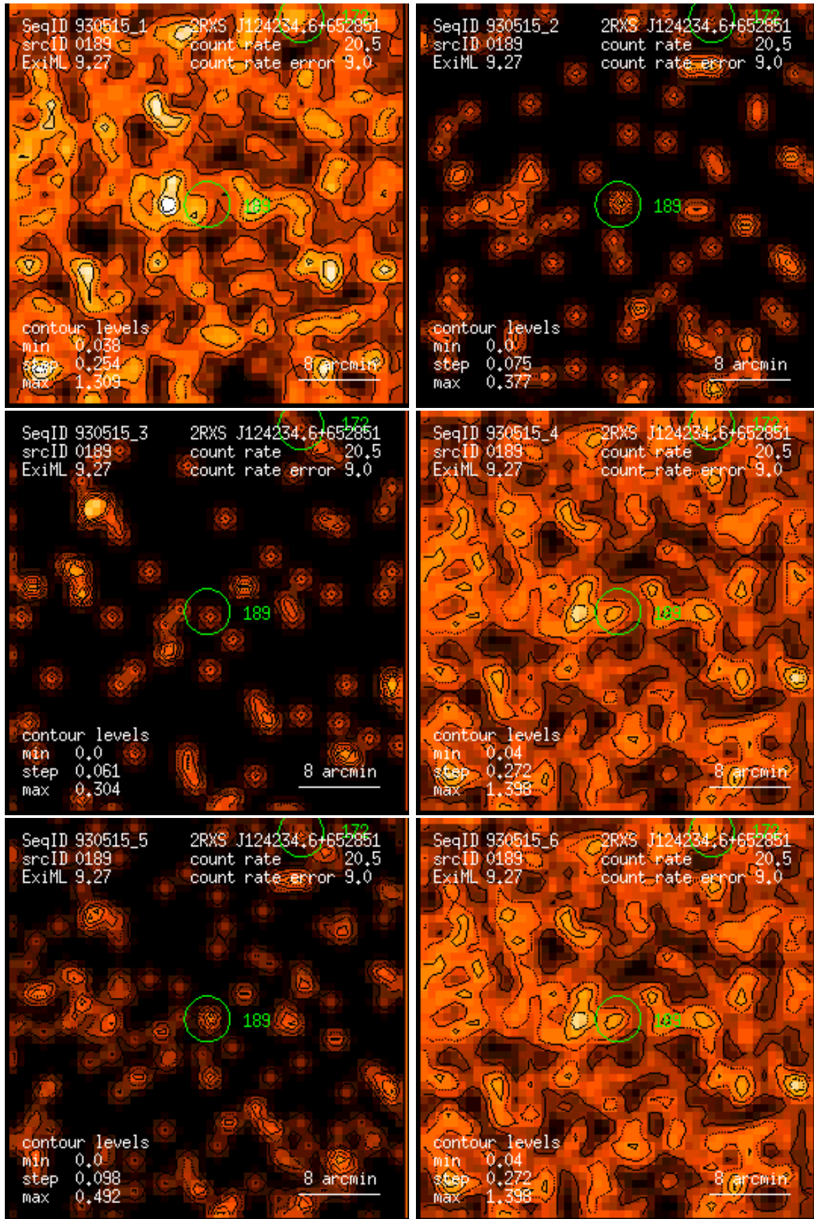
Figure 189: RASS 930515: detection 0189: band rate images, Gaussian filter: (1) PSPC channels 11 – 41, (2) 52 – 90, (3) 91 – 201, (4) 11 – 235, (5) 52 – 201, (6) 11 – 201. Broad band rates in counts/ks. Band rate contour levels in counts/ks/arcmin 2 .
