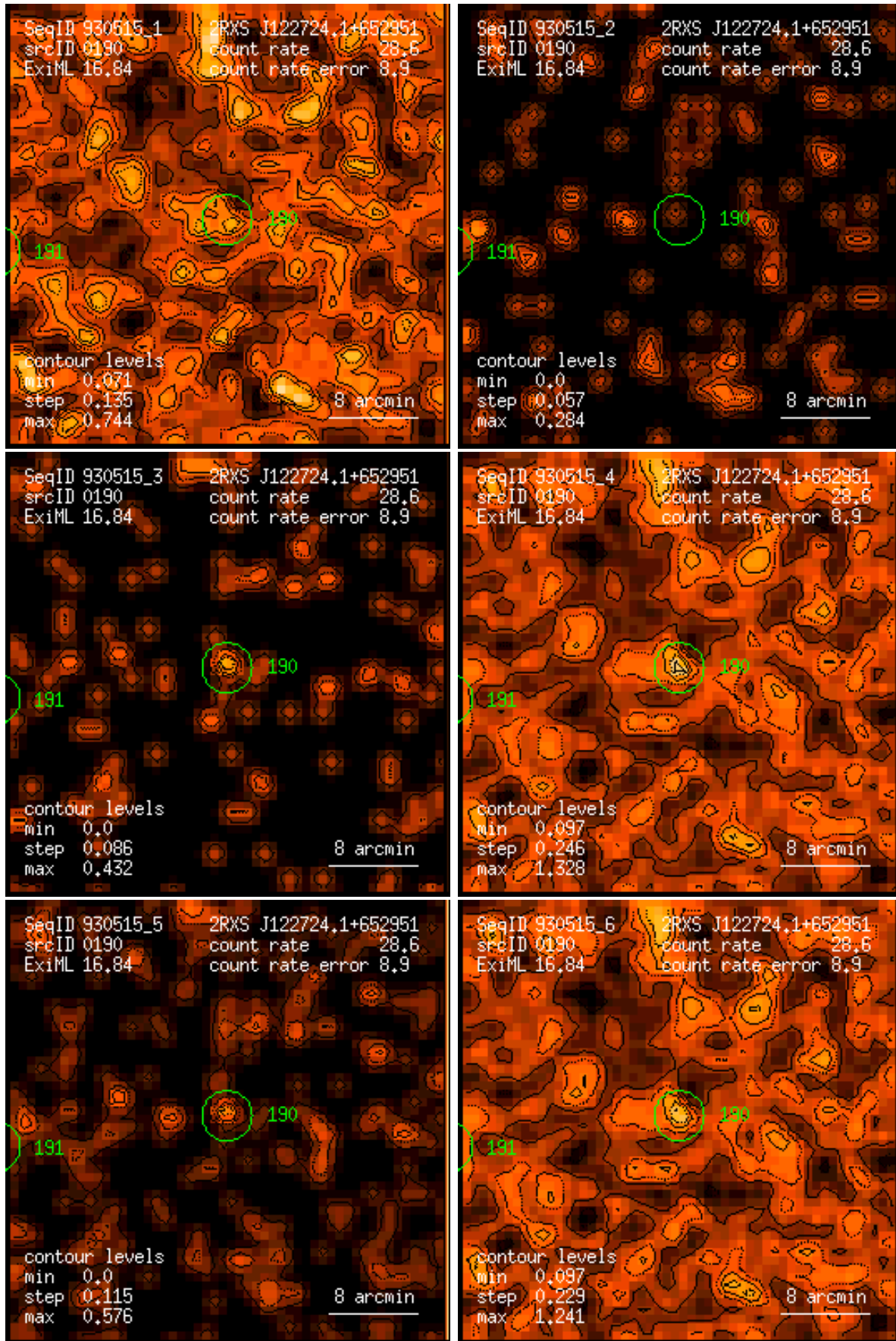
Figure 190: RASS 930515: detection 0190: band rate images, Gaussian filter: (1) PSPC channels 11 – 41, (2) 52 – 90, (3) 91 – 201, (4) 11 – 235, (5) 52 – 201, (6) 11 – 201. Broad band rates in counts/ks. Band rate contour levels in counts/ks/arcmin 2 .
