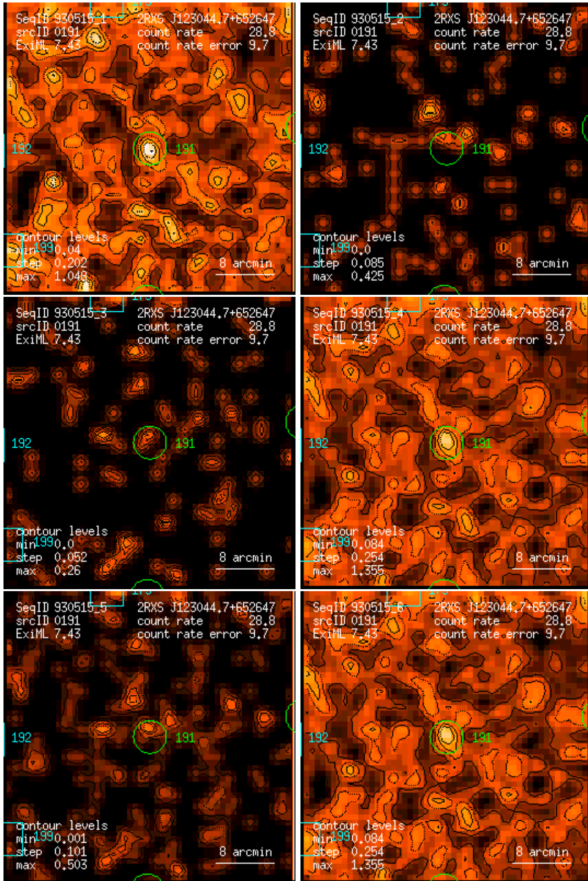
Figure 191: RASS 930515: detection 0191: band rate images, Gaussian filter: (1) PSPC channels 11 – 41, (2) 52 – 90, (3) 91 – 201, (4) 11 – 235, (5) 52 – 201, (6) 11 – 201. Broad band rates in counts/ks. Band rate contour levels in counts/ks/arcmin 2 .
