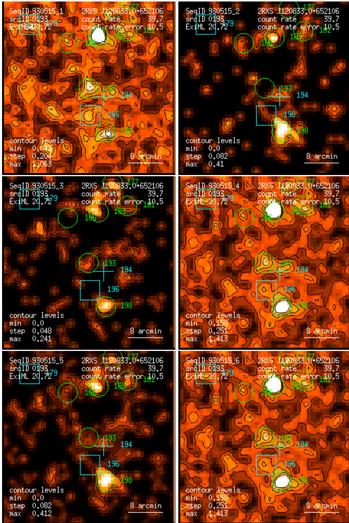
Figure 193: RASS 930515: detection 0193: band rate images, Gaussian filter: (1) PSPC channels 11 – 41, (2) 52 – 90, (3) 91 – 201, (4) 11 – 235, (5) 52 – 201, (6) 11 – 201. Broad band rates in counts/ks. Band rate contour levels in counts/ks/arcmin 2 .
