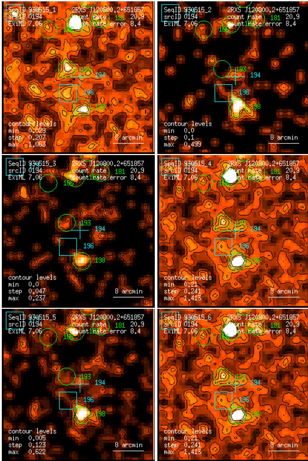
Figure 194: RASS 930515: detection 0194: band rate images, Gaussian filter: (1) PSPC channels 11 – 41, (2) 52 – 90, (3) 91 – 201, (4) 11 – 235, (5) 52 – 201, (6) 11 – 201. Broad band rates in counts/ks. Band rate contour levels in counts/ks/arcmin 2 .
