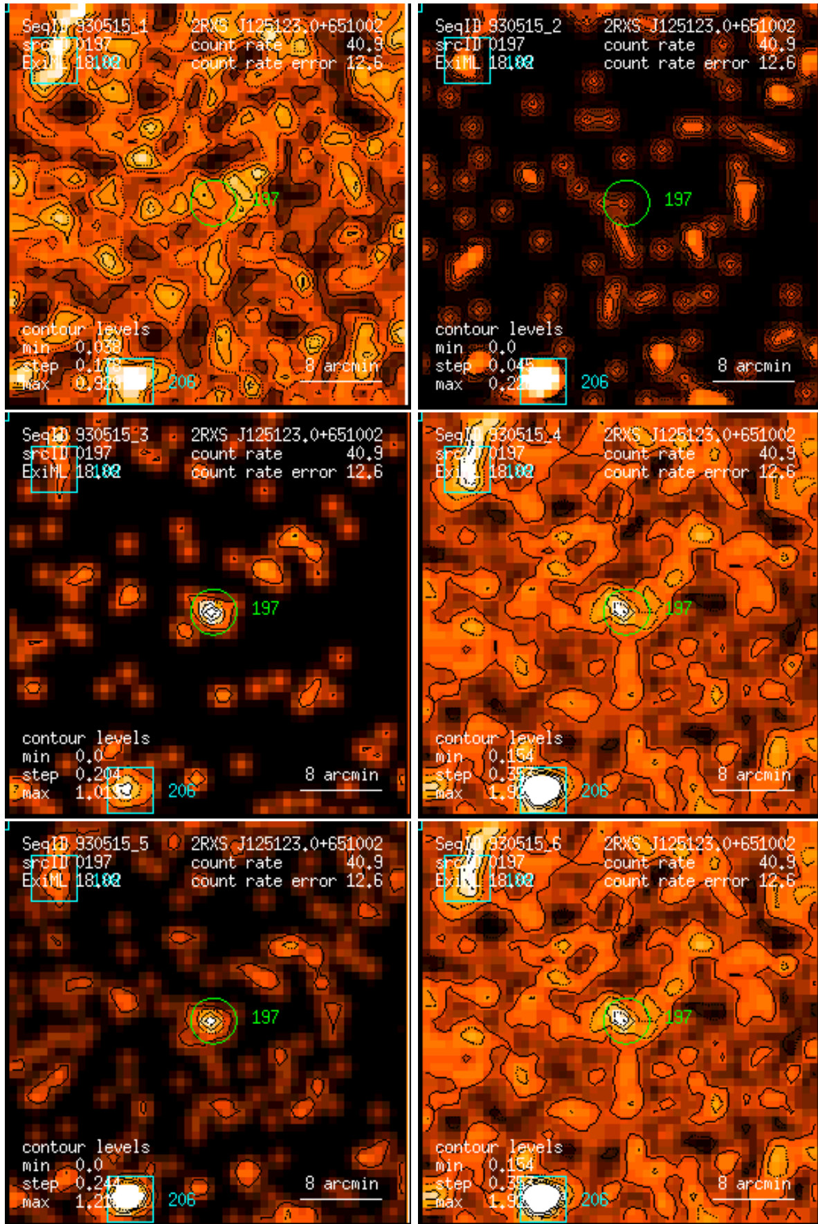
Figure 197: RASS 930515: detection 0197: band rate images, Gaussian filter: (1) PSPC channels 11 – 41, (2) 52 – 90, (3) 91 – 201, (4) 11 – 235, (5) 52 – 201, (6) 11 – 201. Broad band rates in counts/ks. Band rate contour levels in counts/ks/arcmin 2 .
