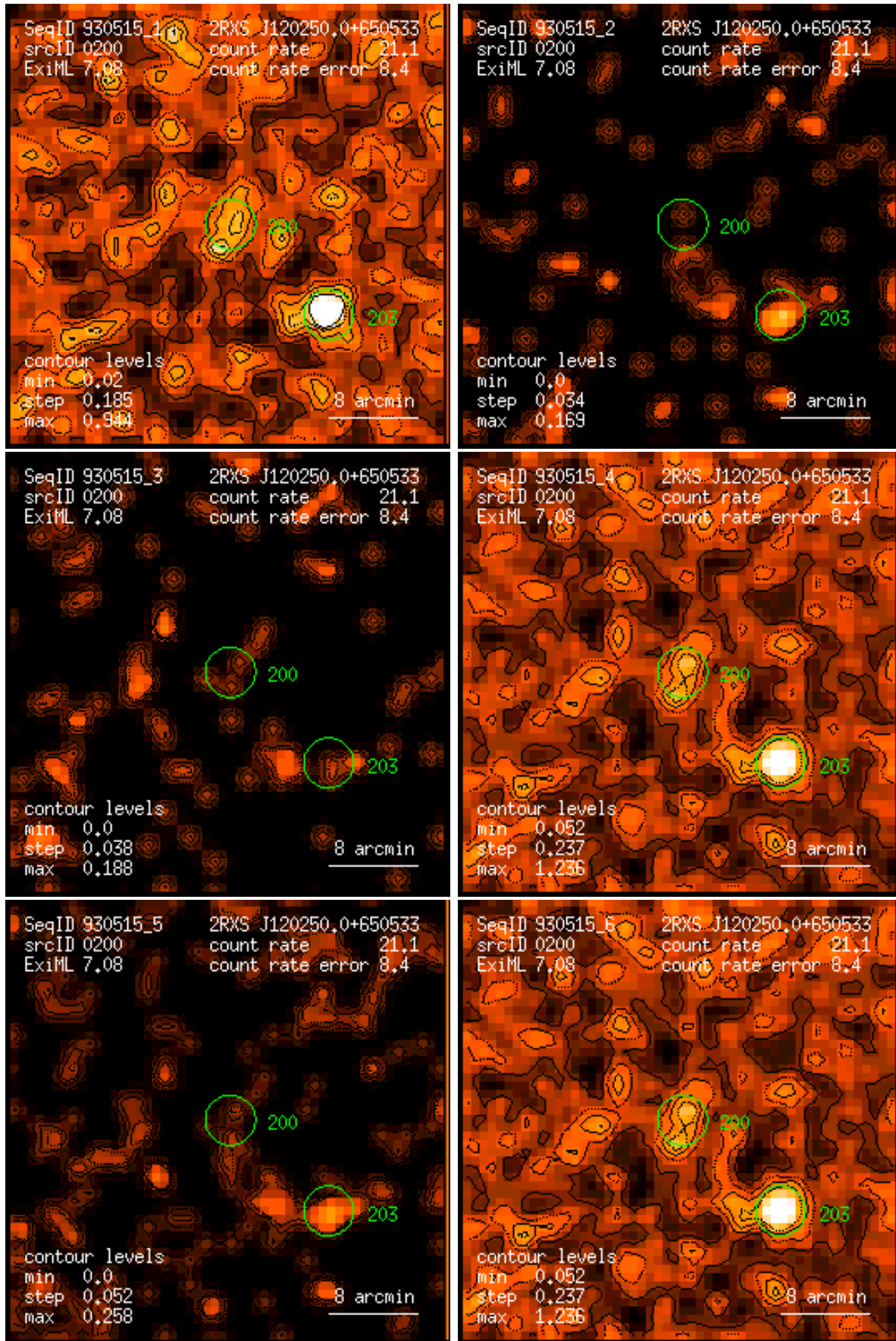
Figure 200: RASS 930515: detection 0200: band rate images, Gaussian filter: (1) PSPC channels 11 – 41, (2) 52 – 90, (3) 91 – 201, (4) 11 – 235, (5) 52 – 201, (6) 11 – 201. Broad band rates in counts/ks. Band rate contour levels in counts/ks/arcmin 2 .
