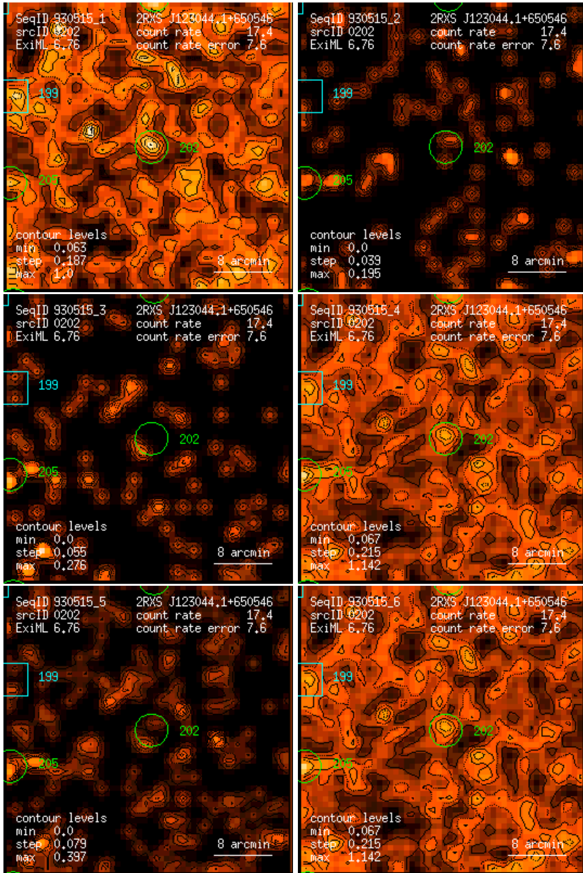
Figure 202: RASS 930515: detection 0202: band rate images, Gaussian filter: (1) PSPC channels 11 – 41, (2) 52 – 90, (3) 91 – 201, (4) 11 – 235, (5) 52 – 201, (6) 11 – 201. Broad band rates in counts/ks. Band rate contour levels in counts/ks/arcmin 2 .
