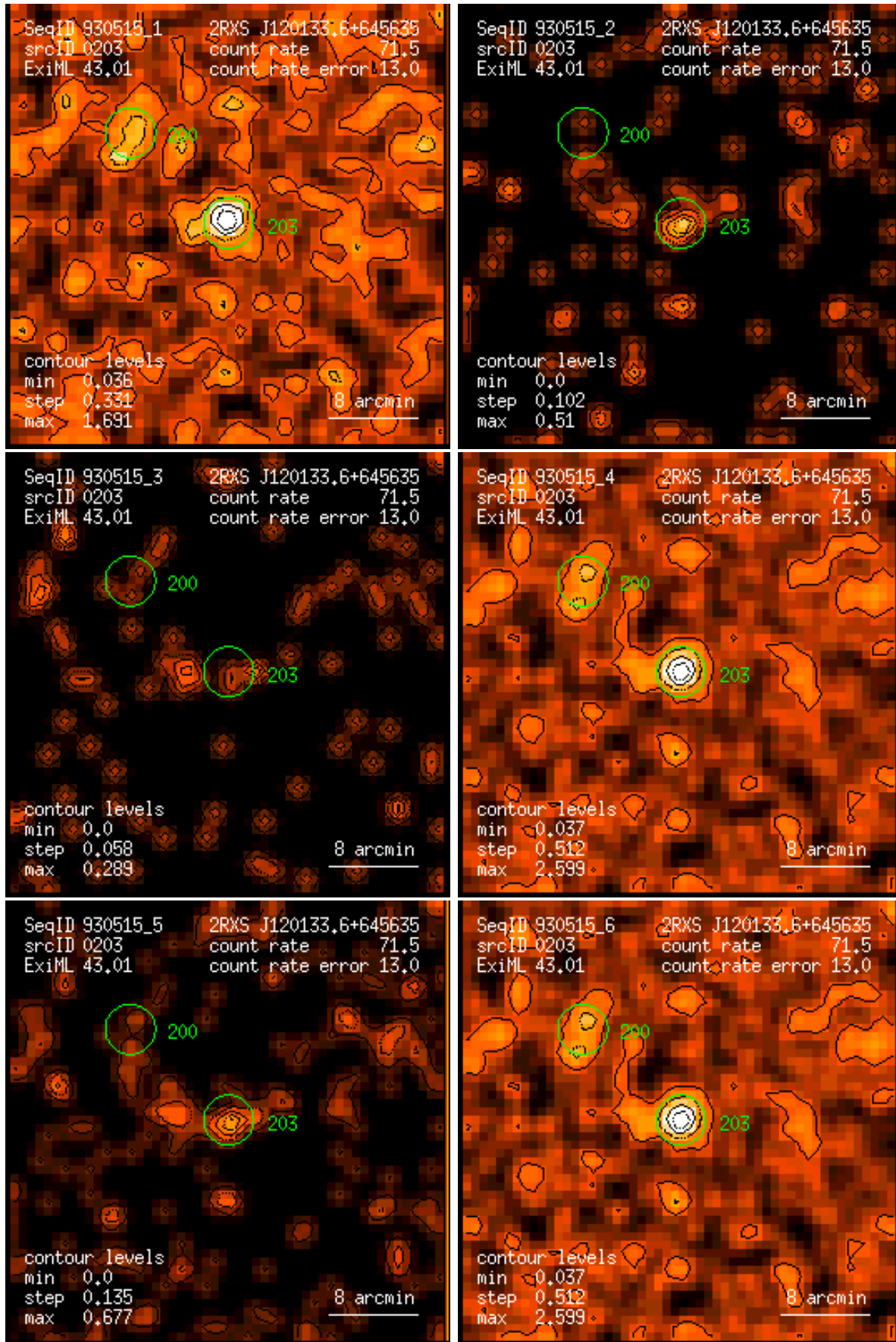
Figure 203: RASS 930515: detection 0203: band rate images, Gaussian filter: (1) PSPC channels 11 – 41, (2) 52 – 90, (3) 91 – 201, (4) 11 – 235, (5) 52 – 201, (6) 11 – 201. Broad band rates in counts/ks. Band rate contour levels in counts/ks/arcmin 2 .
