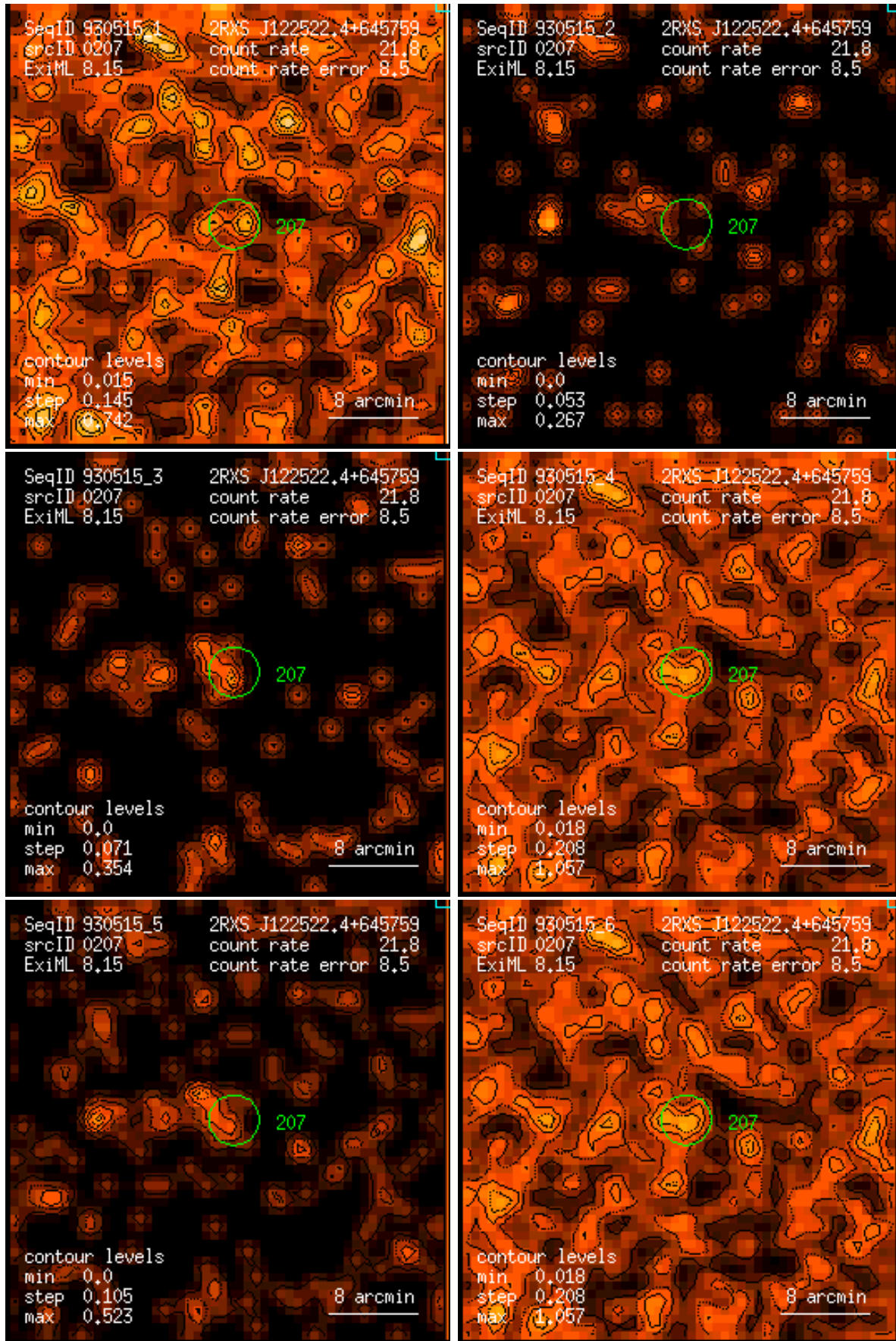
Figure 207: RASS 930515: detection 0207: band rate images, Gaussian filter: (1) PSPC channels 11 – 41, (2) 52 – 90, (3) 91 – 201, (4) 11 – 235, (5) 52 – 201, (6) 11 – 201. Broad band rates in counts/ks. Band rate contour levels in counts/ks/arcmin 2 .
