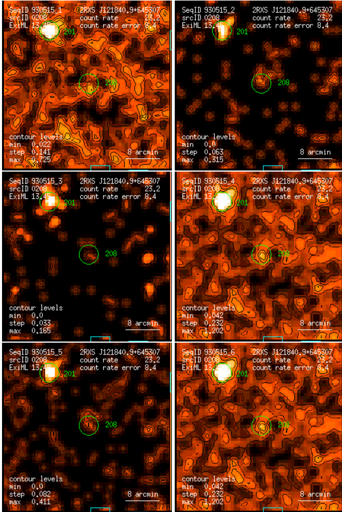
Figure 208: RASS 930515: detection 0208: band rate images, Gaussian filter: (1) PSPC channels 11 – 41, (2) 52 – 90, (3) 91 – 201, (4) 11 – 235, (5) 52 – 201, (6) 11 – 201. Broad band rates in counts/ks. Band rate contour levels in counts/ks/arcmin 2 .
