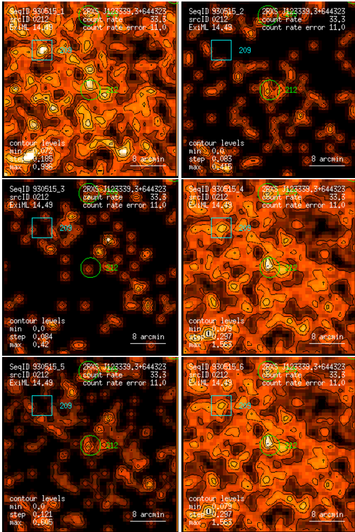
Figure 212: RASS 930515: detection 0212: band rate images, Gaussian filter: (1) PSPC channels 11 – 41, (2) 52 – 90, (3) 91 – 201, (4) 11 – 235, (5) 52 – 201, (6) 11 – 201. Broad band rates in counts/ks. Band rate contour levels in counts/ks/arcmin 2 .
