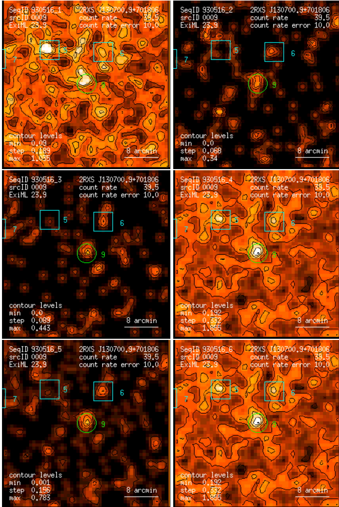
Figure 9: RASS 930516: detection 0009: band rate images, Gaussian filter: (1) PSPC channels 11 – 41, (2) 52 – 90, (3) 91 – 201, (4) 11 – 235, (5) 52 – 201, (6) 11 – 201. Broad band rates in counts/ks. Band rate contour levels in counts/ks/arcmin 2 .
