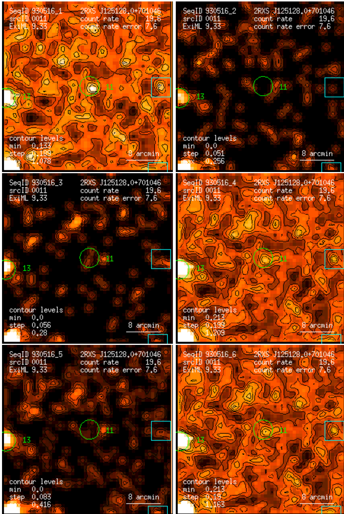
Figure 11: RASS 930516: detection 0011: band rate images, Gaussian filter: (1) PSPC channels 11 – 41, (2) 52 – 90, (3) 91 – 201, (4) 11 – 235, (5) 52 – 201, (6) 11 – 201. Broad band rates in counts/ks. Band rate contour levels in counts/ks/arcmin 2 .
