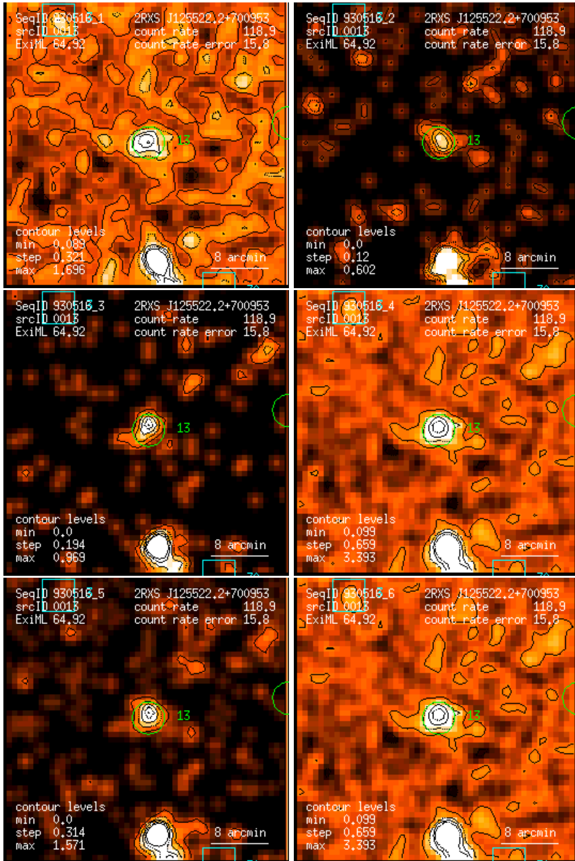
Figure 13: RASS 930516: detection 0013: band rate images, Gaussian filter: (1) PSPC channels 11 – 41, (2) 52 – 90, (3) 91 – 201, (4) 11 – 235, (5) 52 – 201, (6) 11 – 201. Broad band rates in counts/ks. Band rate contour levels in counts/ks/arcmin 2 .
