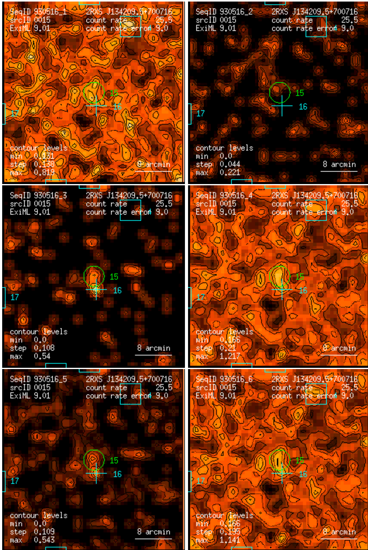
Figure 15: RASS 930516: detection 0015: band rate images, Gaussian filter: (1) PSPC channels 11 – 41, (2) 52 – 90, (3) 91 – 201, (4) 11 – 235, (5) 52 – 201, (6) 11 – 201. Broad band rates in counts/ks. Band rate contour levels in counts/ks/arcmin 2 .
